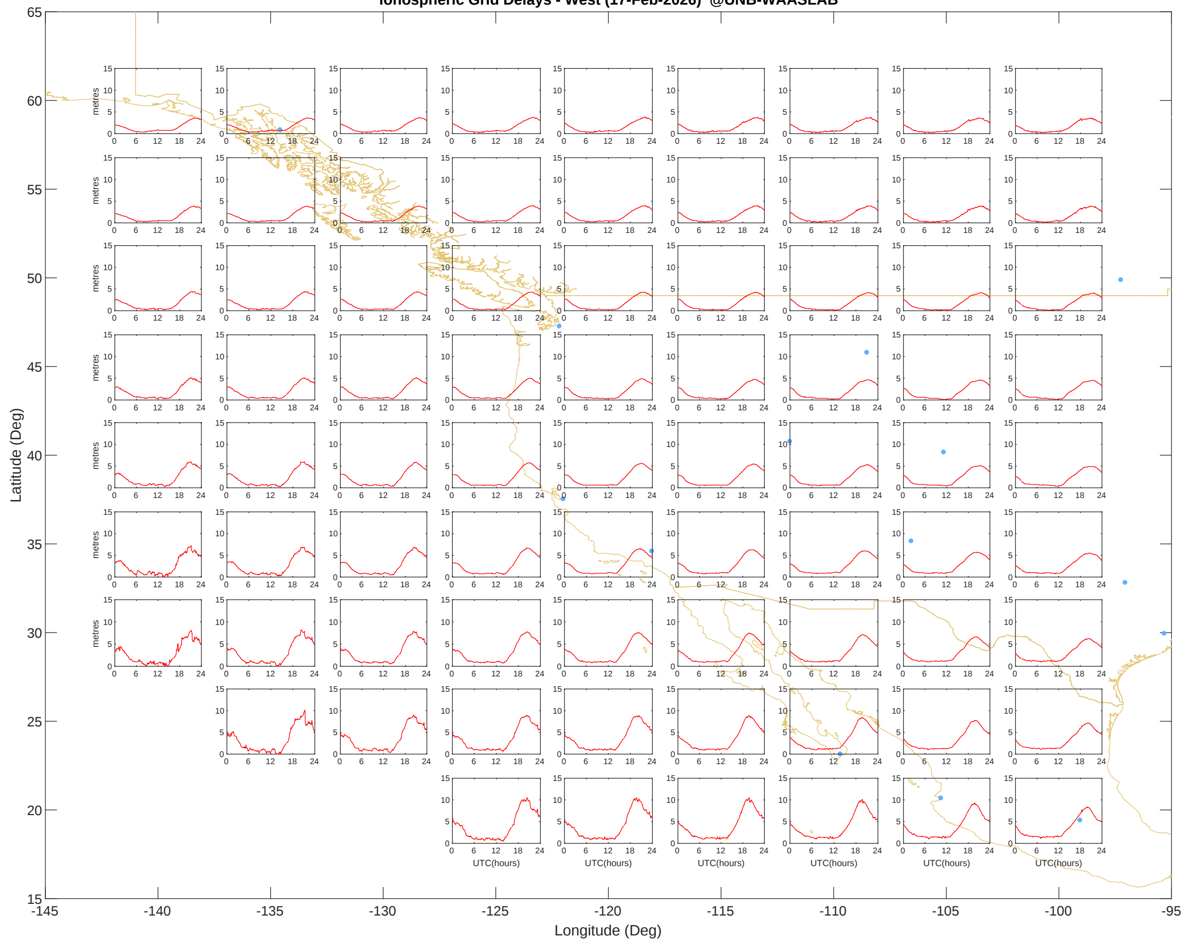
Ionospheric Grid Delays - West (17-Feb-2026) @UNB-WAASLAB
