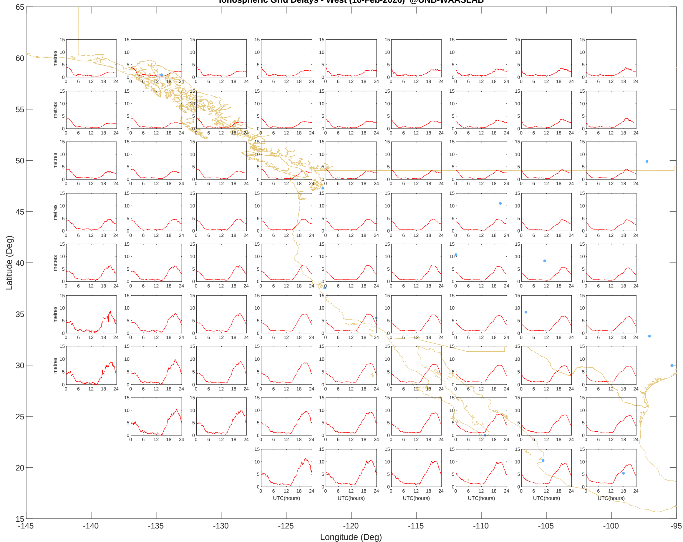
Ionospheric Grid Delays - West (16-Feb-2026) @UNB-WAASLAB
