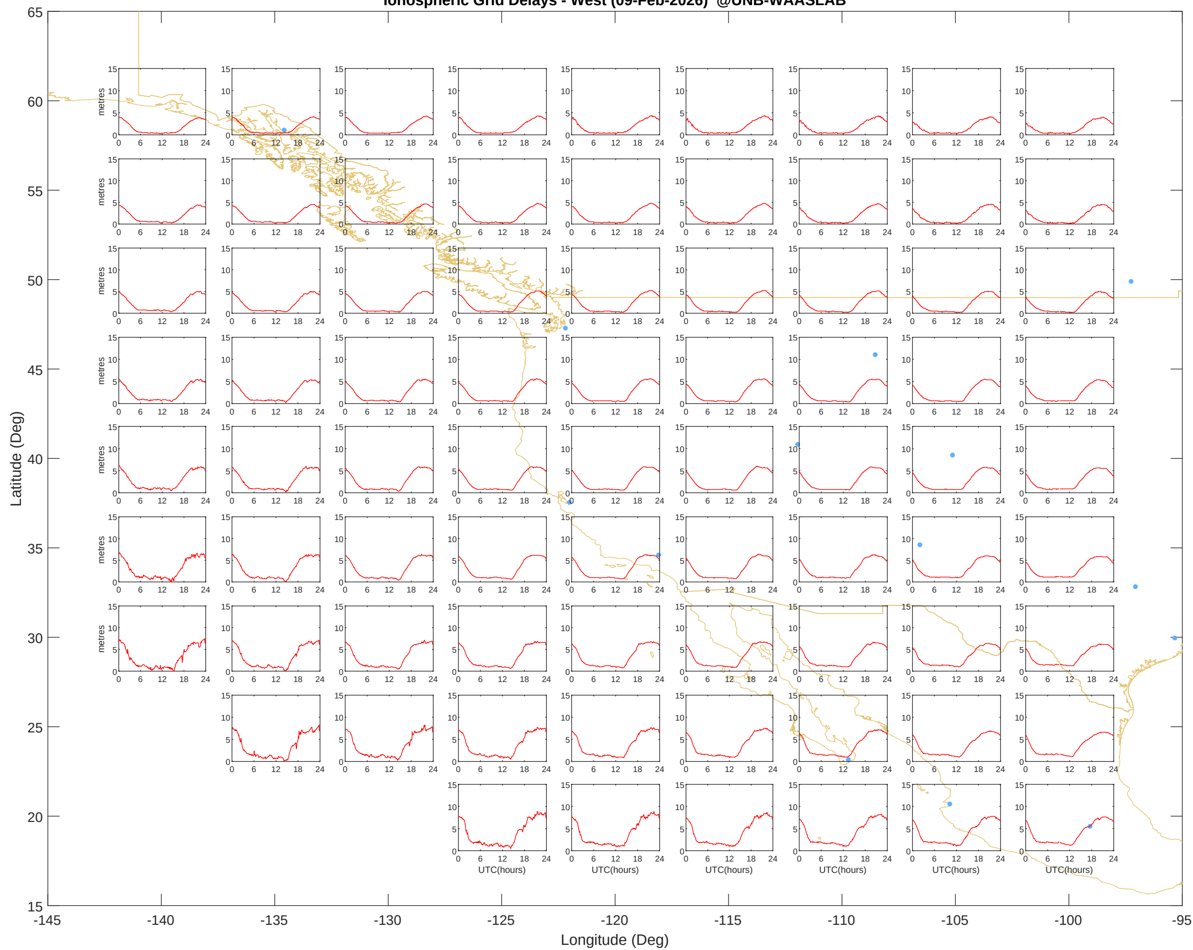
Ionospheric Grid Delays - West (09-Feb-2026) @UNB-WAASLAB
