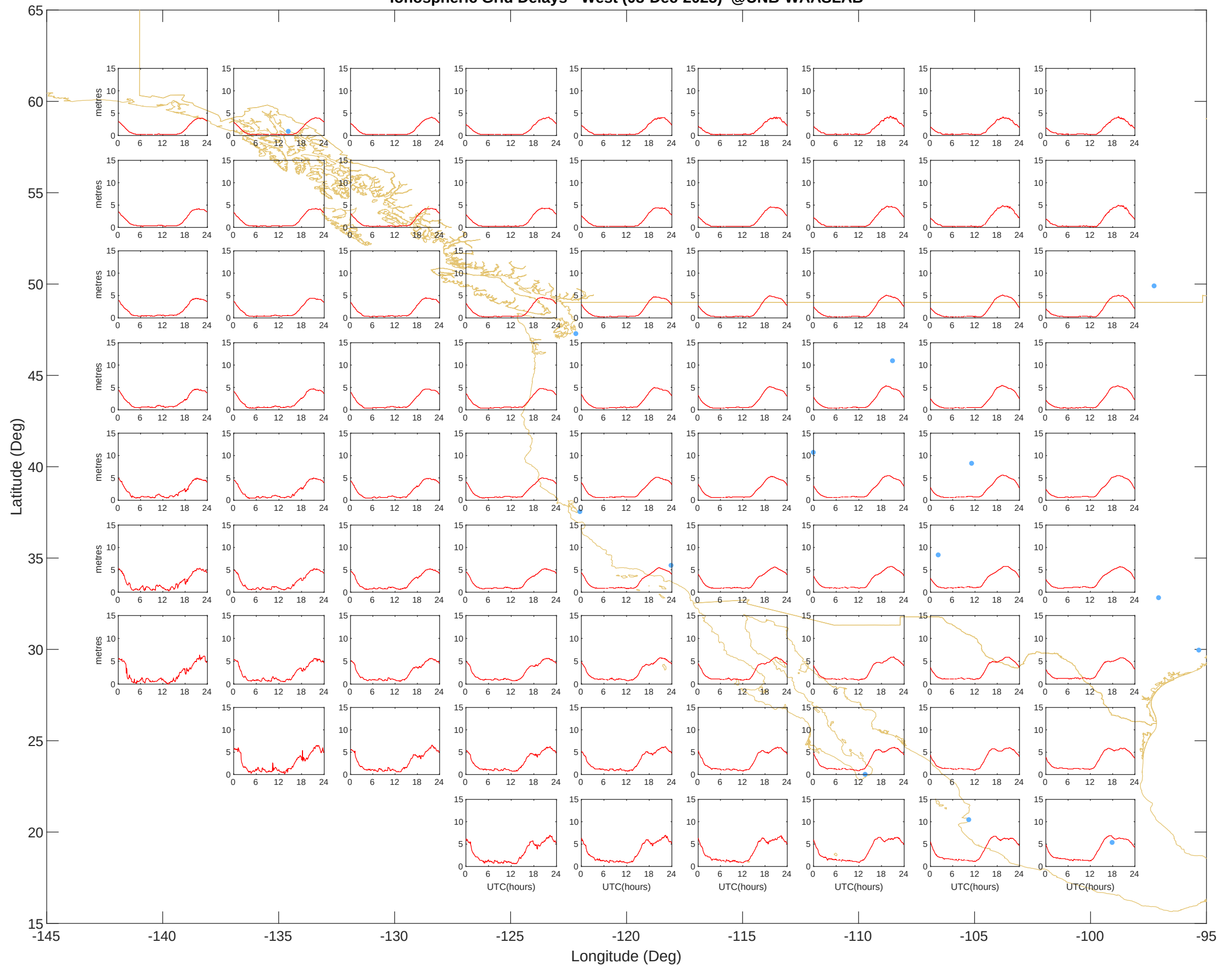
Ionospheric Grid Delays - West (08-Dec-2025) @UNB-WAASLAB
