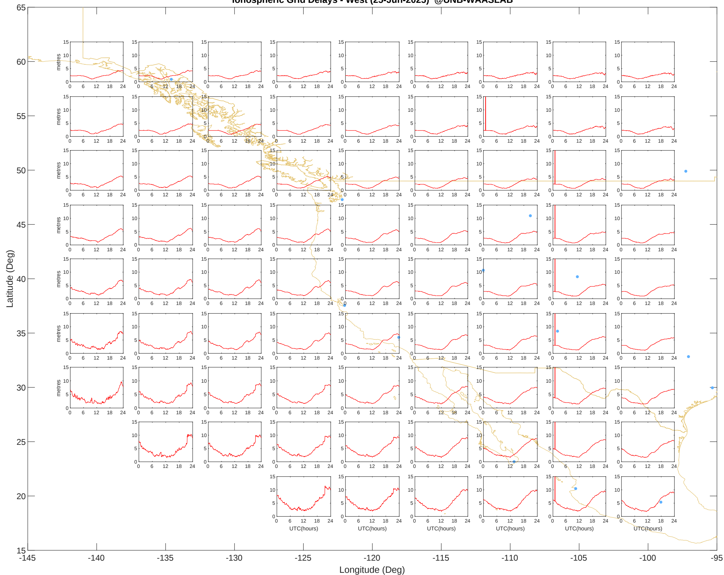
Ionospheric Grid Delays - West (25-Jun-2025) @UNB-WAASLAB
