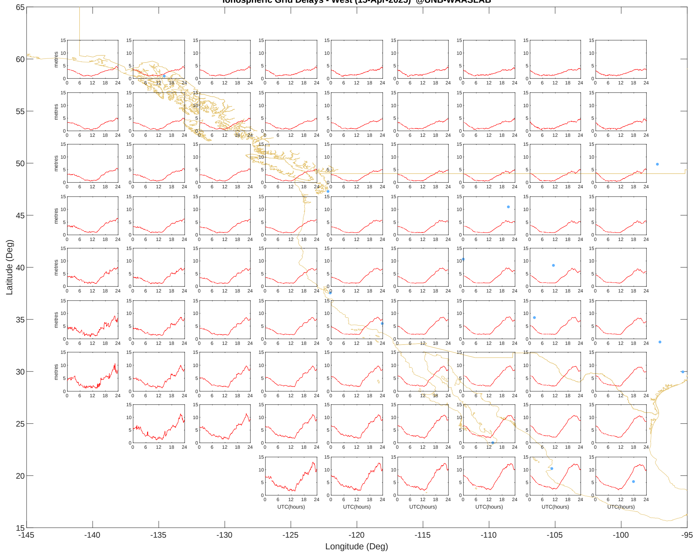
Ionospheric Grid Delays - West (15-Apr-2025) @UNB-WAASLAB
