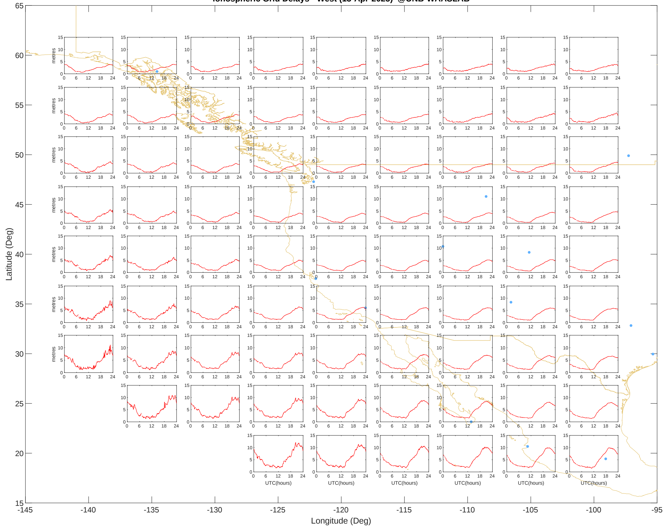
Ionospheric Grid Delays - West (13-Apr-2025) @UNB-WAASLAB
