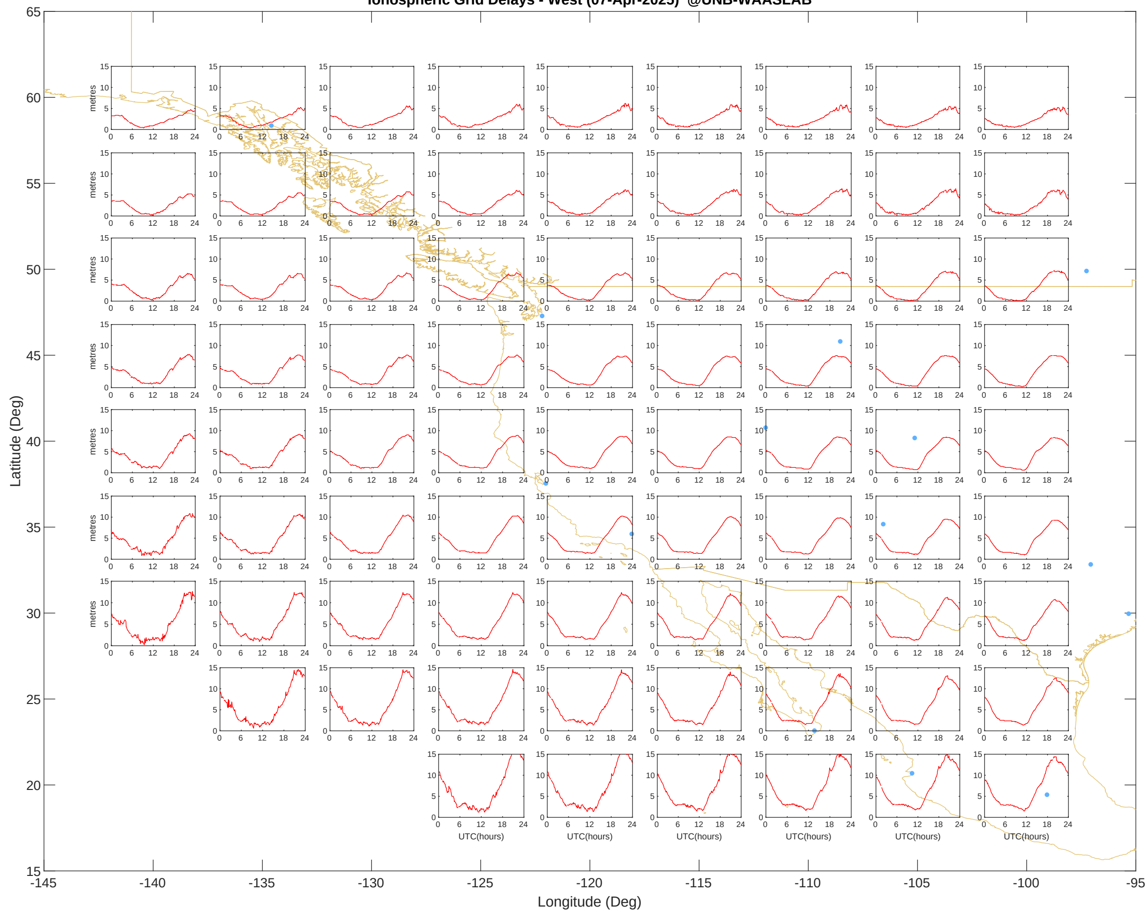
Ionospheric Grid Delays - West (07-Apr-2025) @UNB-WAASLAB
