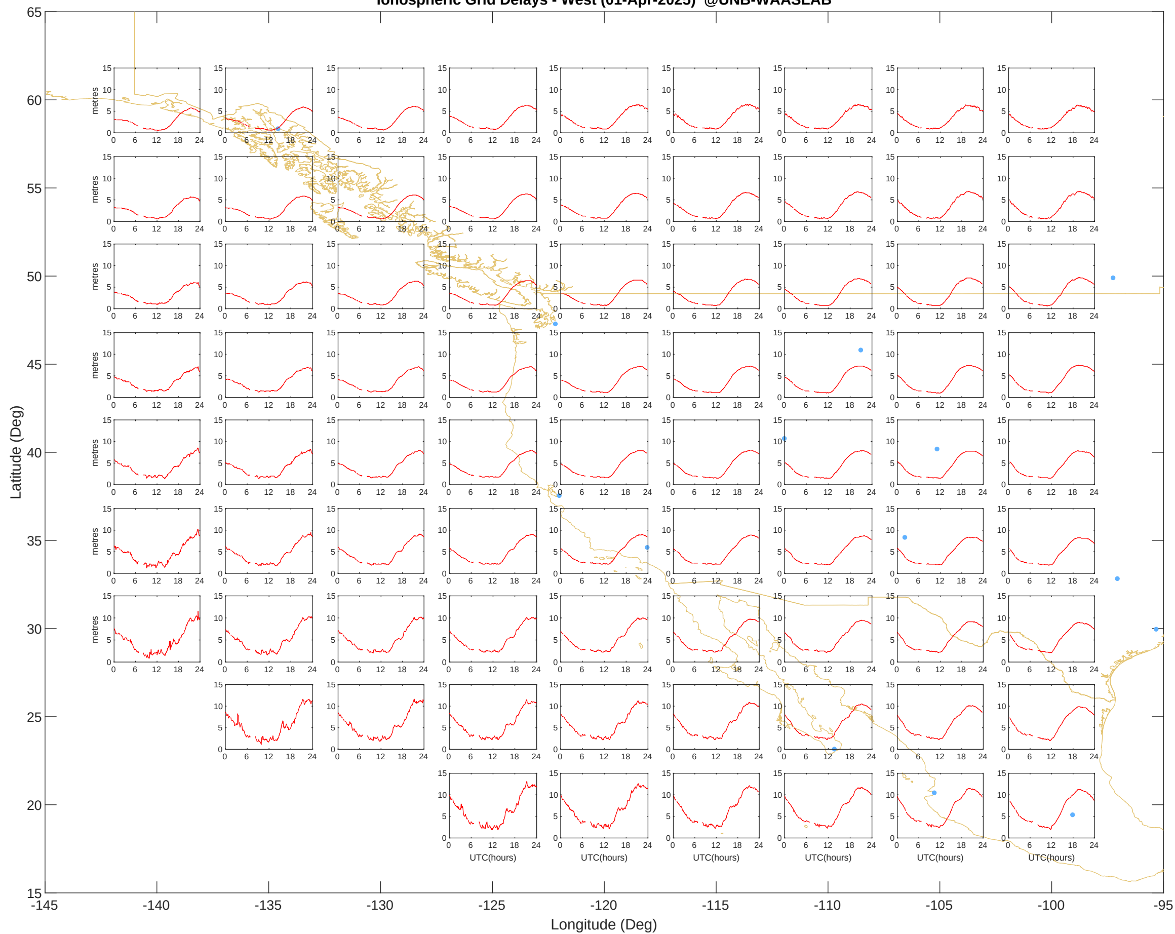
Ionospheric Grid Delays - West (01-Apr-2025) @UNB-WAASLAB
