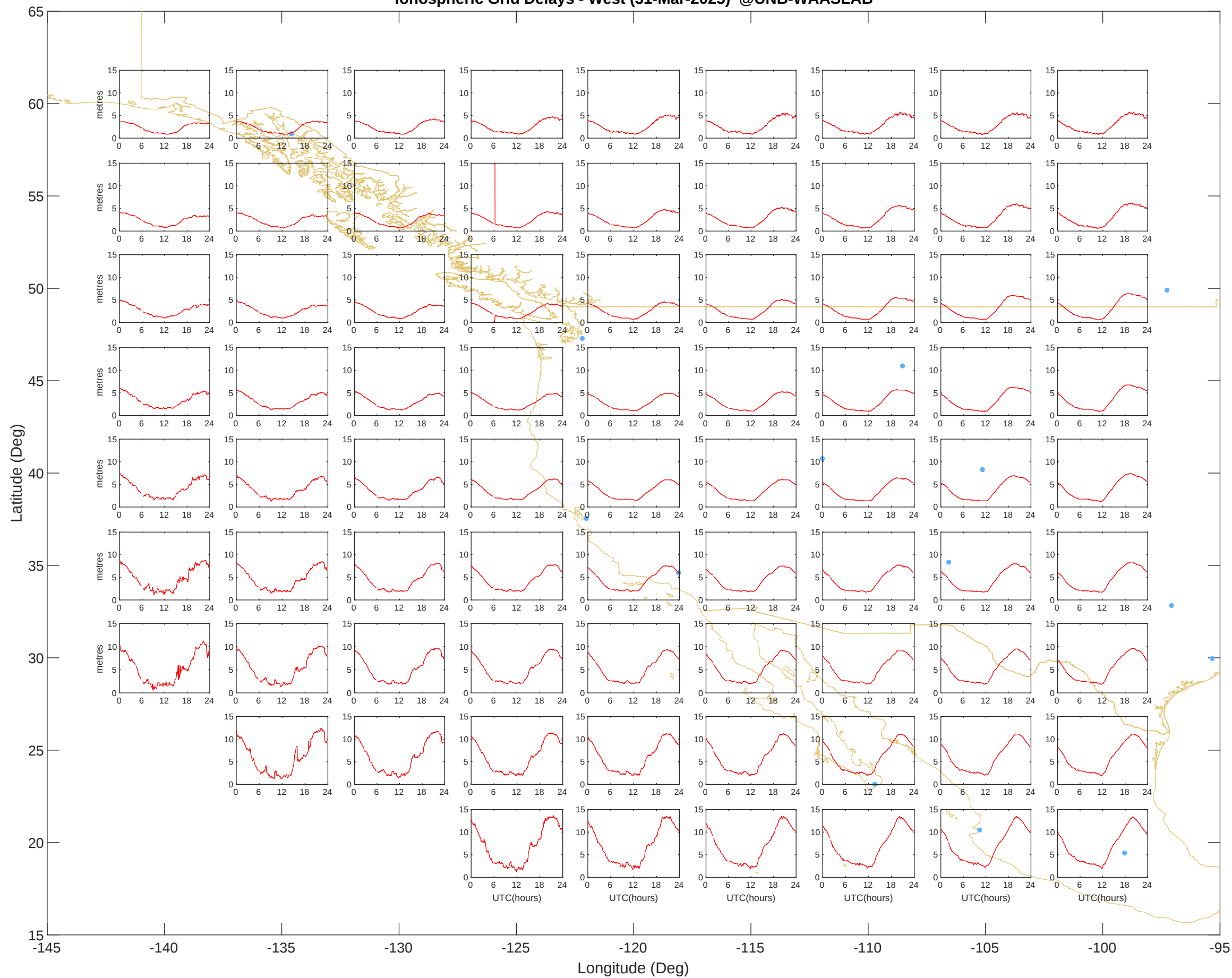
Ionospheric Grid Delays - West (31-Mar-2025) @UNB-WAASLAB
