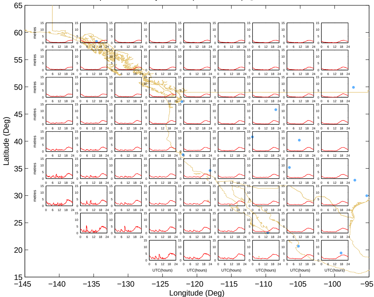
Ionospheric Grid Delays – West (13-Jan-2016) @UNB-WAASLAB
