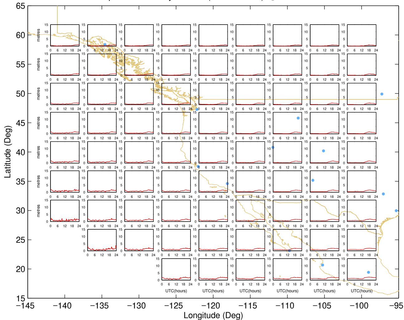
Ionospheric Grid Delays – West (03-Jan-2010) @UNB-WAASLAB
