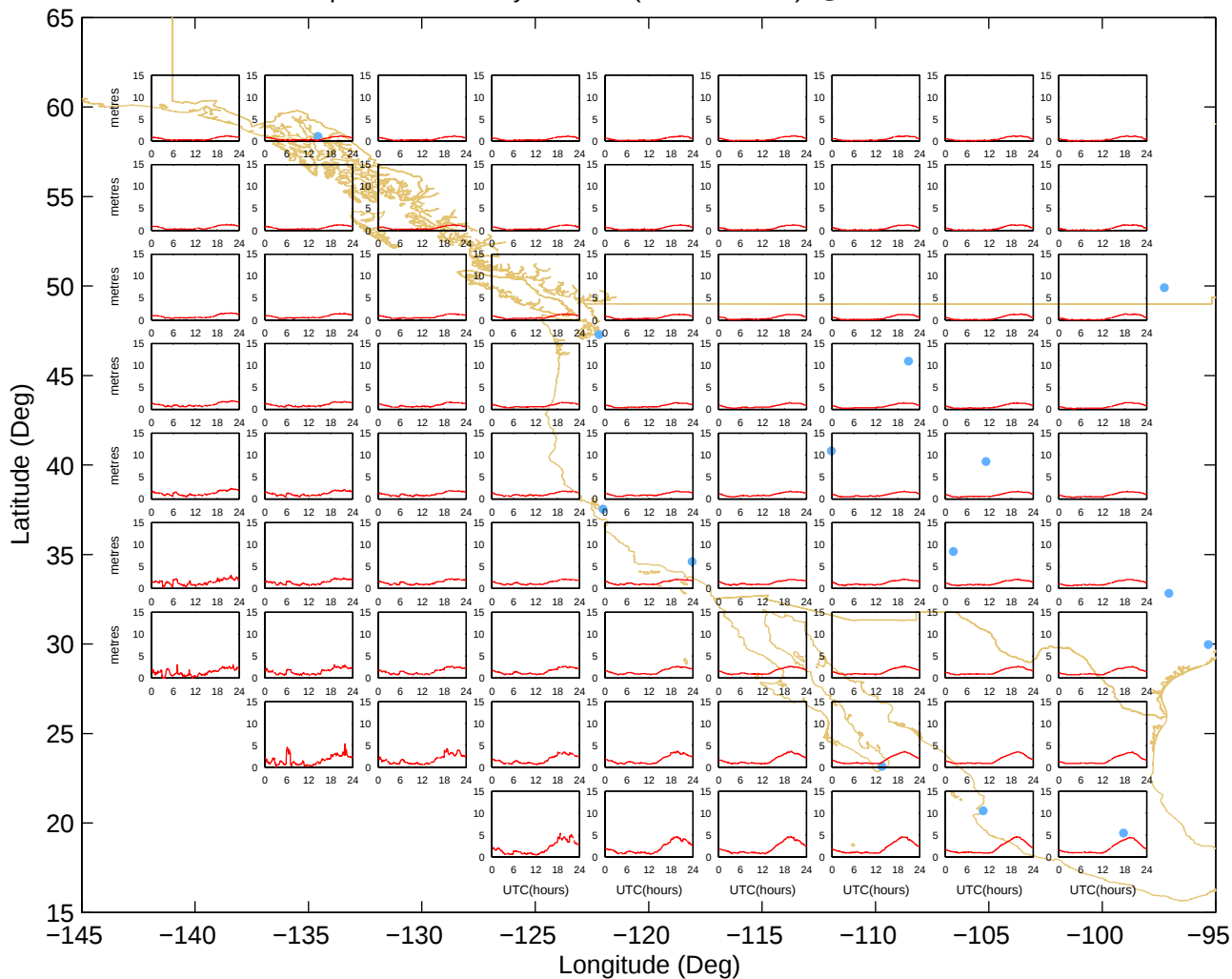
Ionospheric Grid Delays – West (16-Oct-2008) @UNB-WAASLAB
