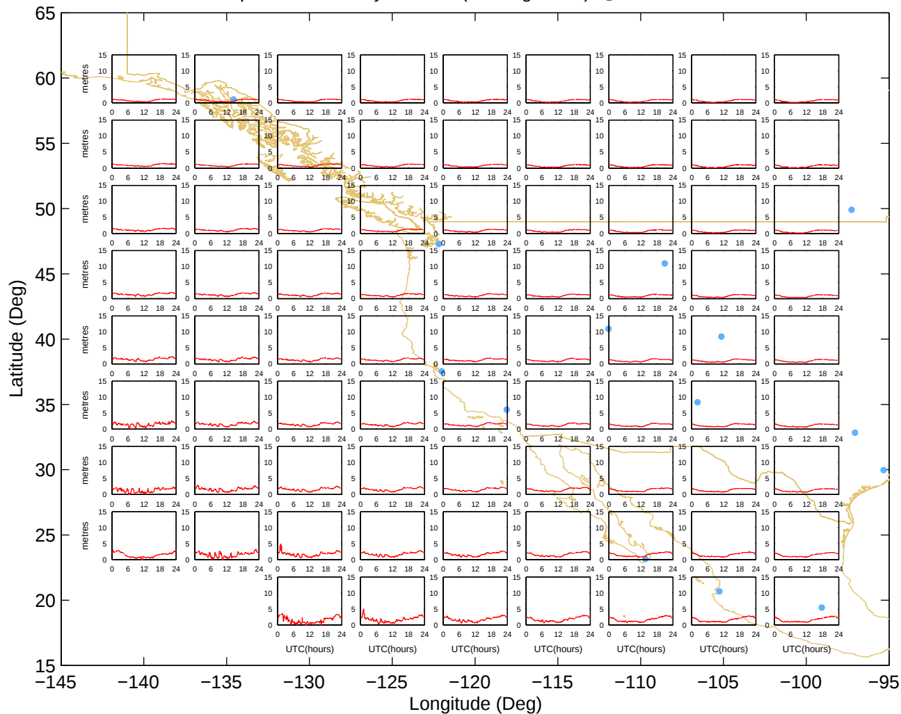
Ionospheric Grid Delays – West (30-Aug-2008) @UNB-WAASLAB
