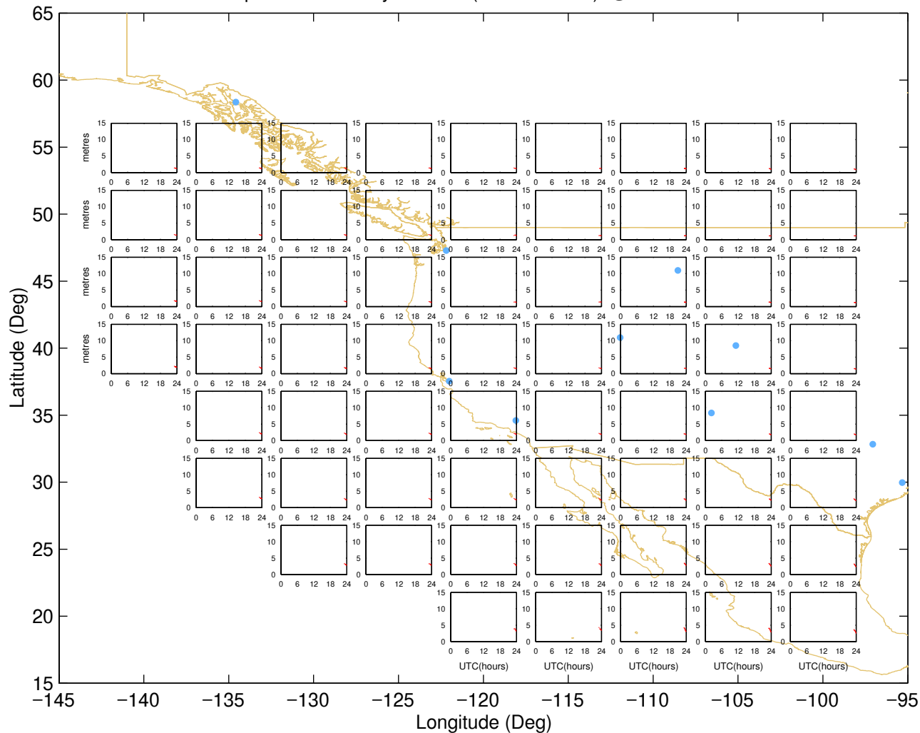
Ionospheric Grid Delays – West (02-Oct-2006) @UNB-WAASLAB
