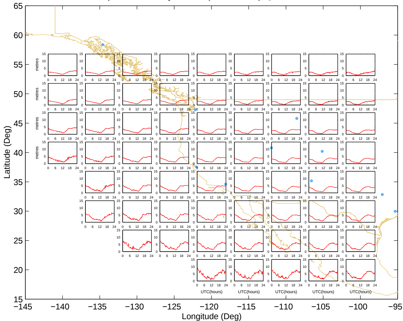
Ionospheric Grid Delays – West (24-Jul-2003) @UNB-WAASLAB
