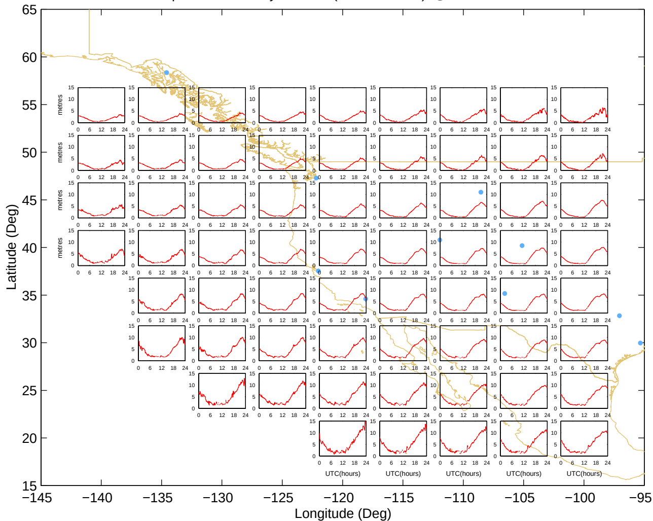
Ionospheric Grid Delays – West (16-Mar-2003) @UNB-WAASLAB
