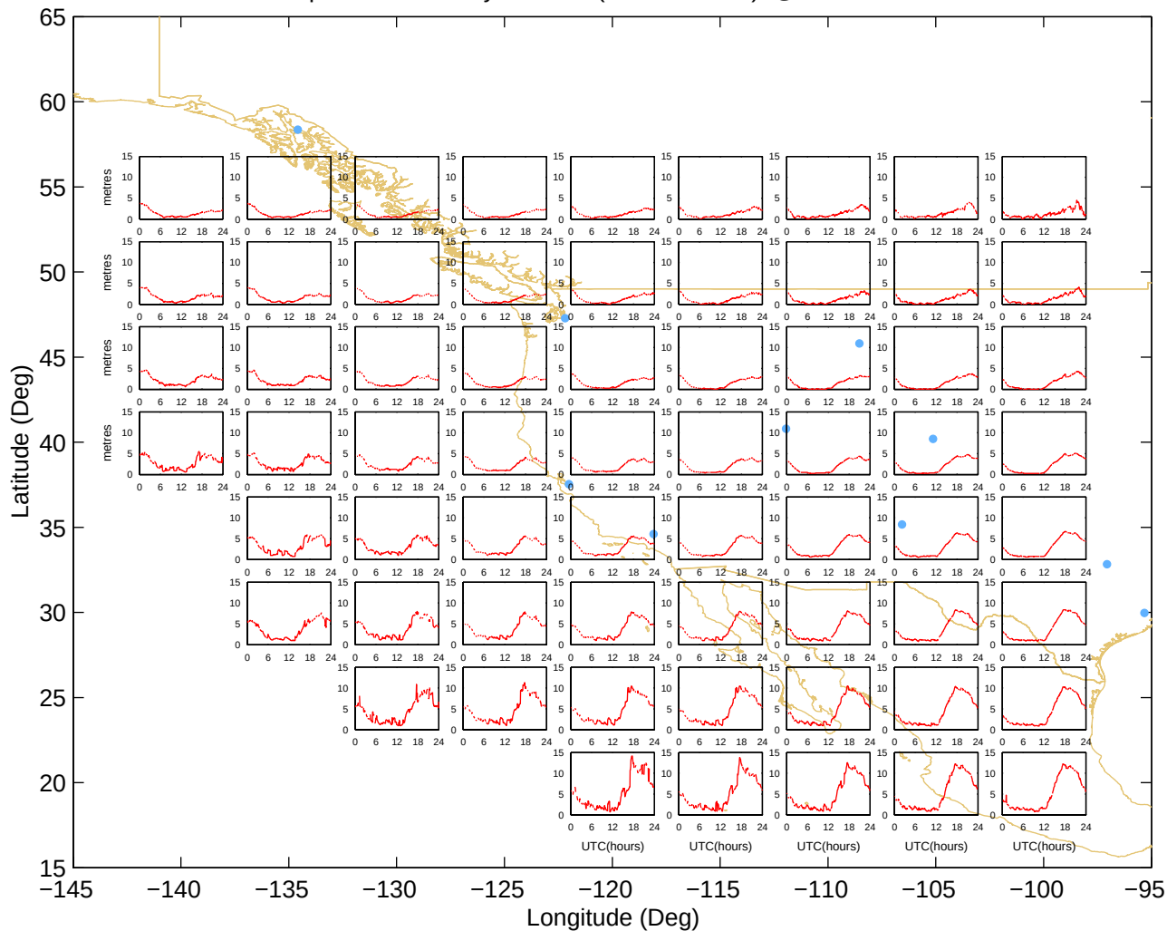
Ionospheric Grid Delays – West (03-Oct-2002) @UNB-WAASLAB
