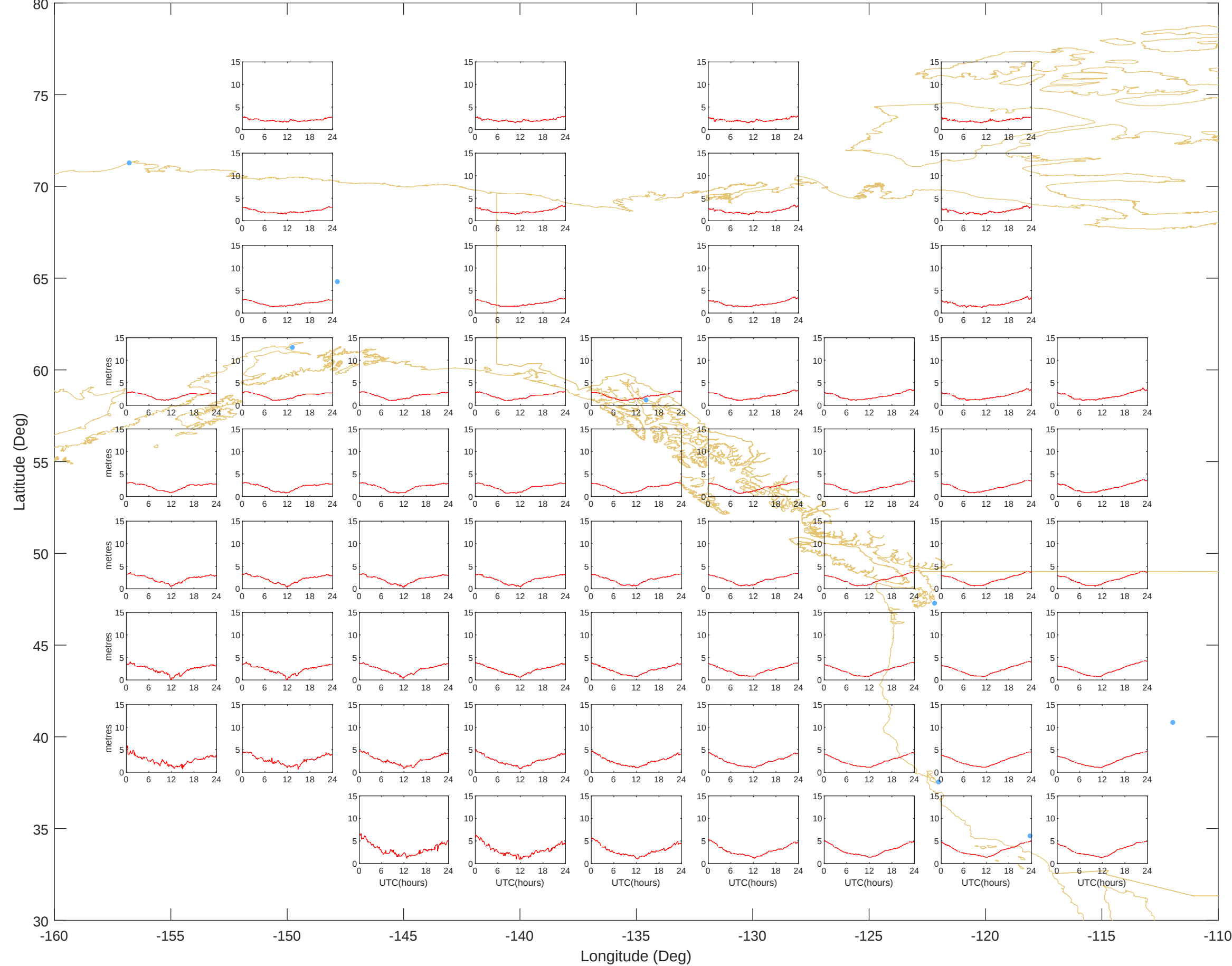
Ionospheric Grid Delays - Alaska (31-May-2025) @UNB-WAASLAB
