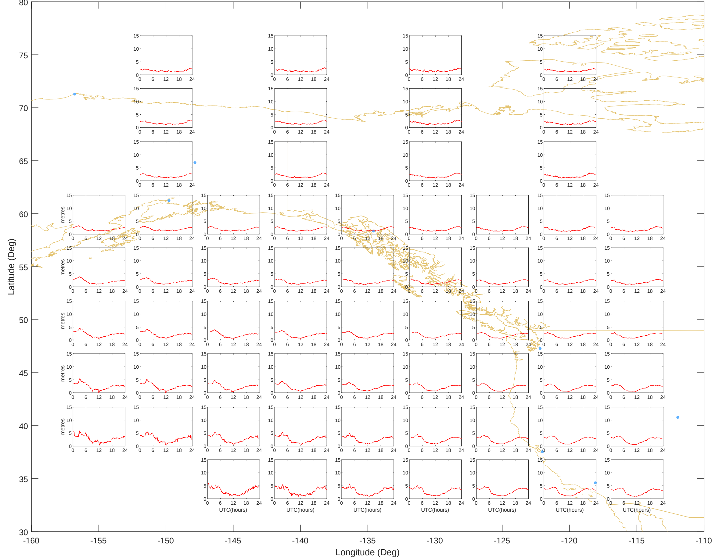
Ionospheric Grid Delays - Alaska (29-May-2025) @UNB-WAASLAB
