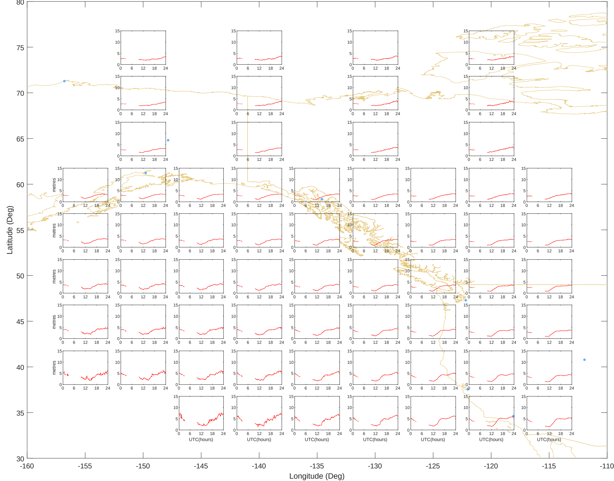
Ionospheric Grid Delays - Alaska (26-May-2025) @UNB-WAASLAB
