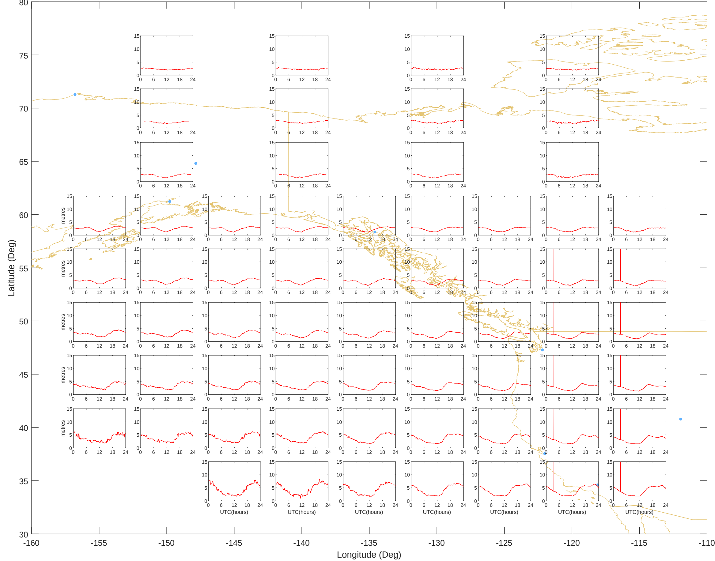
Ionospheric Grid Delays - Alaska (25-May-2025) @UNB-WAASLAB
