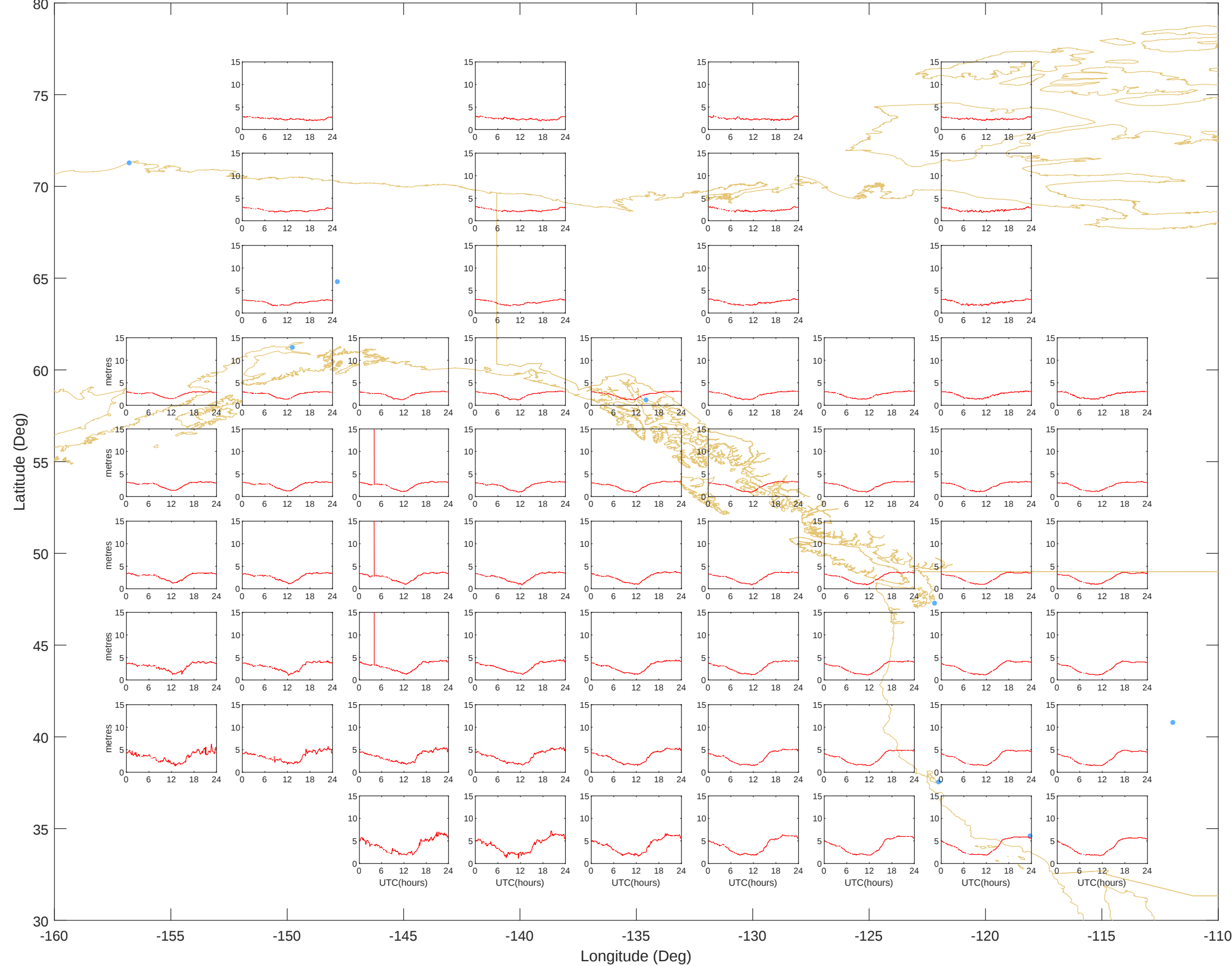
Ionospheric Grid Delays - Alaska (23-May-2025) @UNB-WAASLAB
