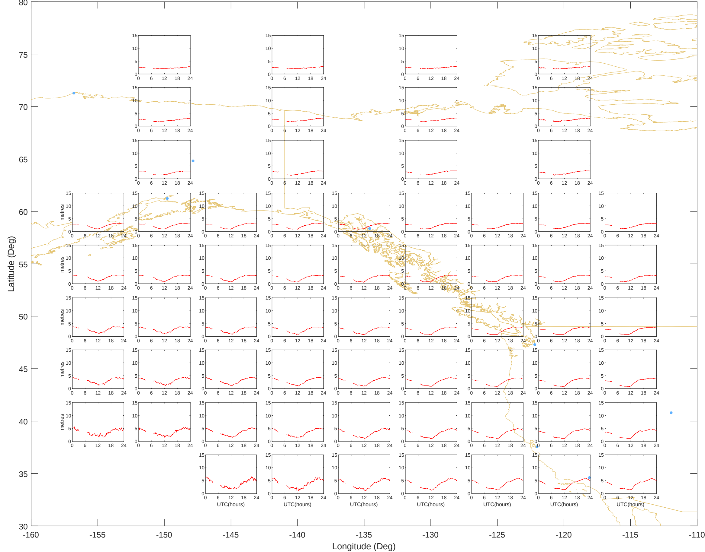
Ionospheric Grid Delays - Alaska (22-May-2025) @UNB-WAASLAB
