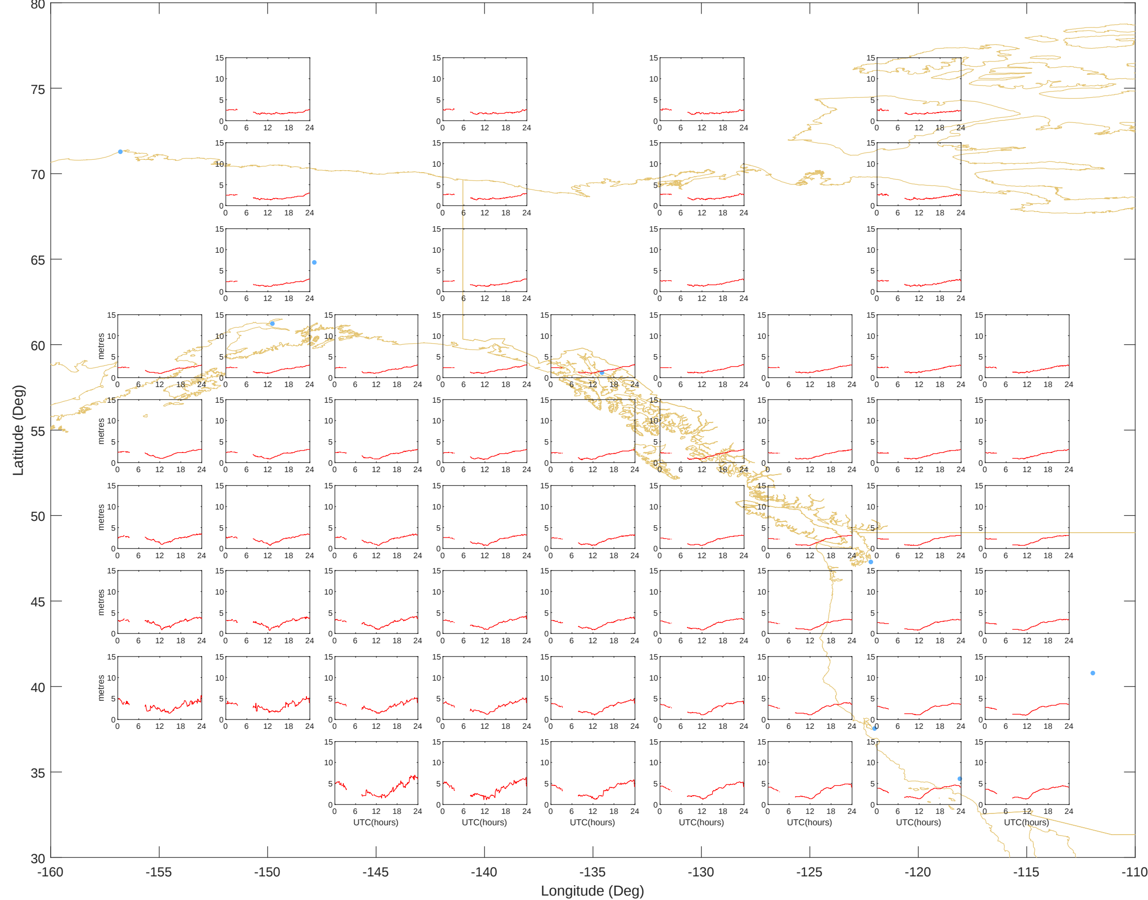
Ionospheric Grid Delays - Alaska (20-May-2025) @UNB-WAASLAB
