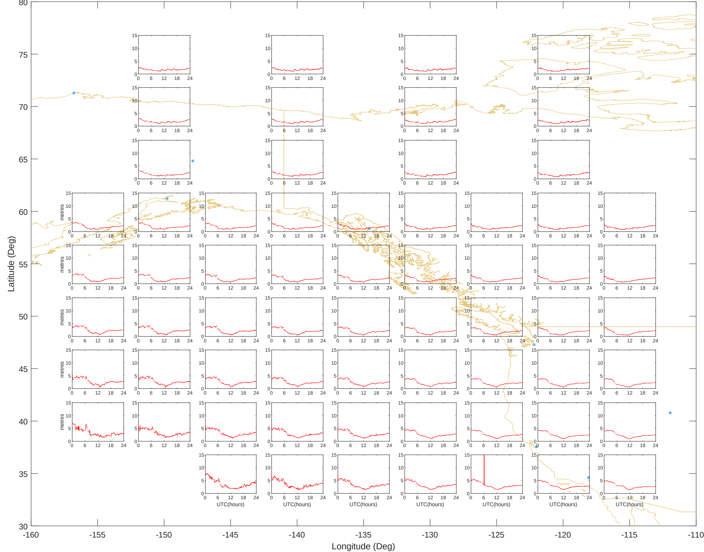
Ionospheric Grid Delays - Alaska (17-May-2025) @UNB-WAASLAB
