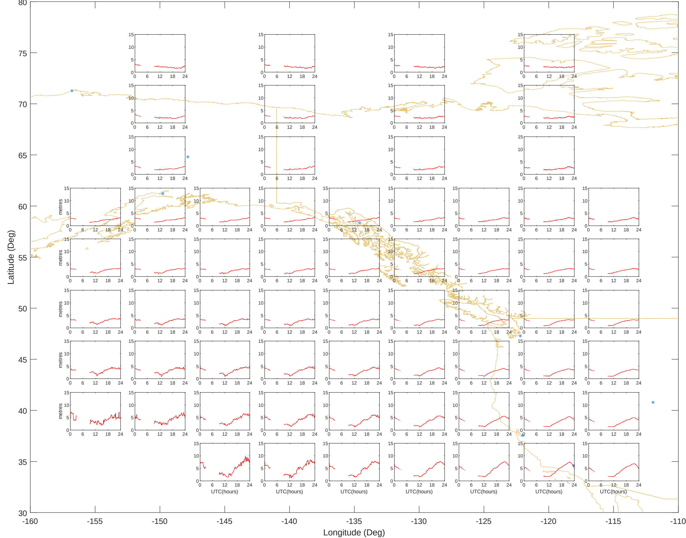
Ionospheric Grid Delays - Alaska (16-May-2025) @UNB-WAASLAB
