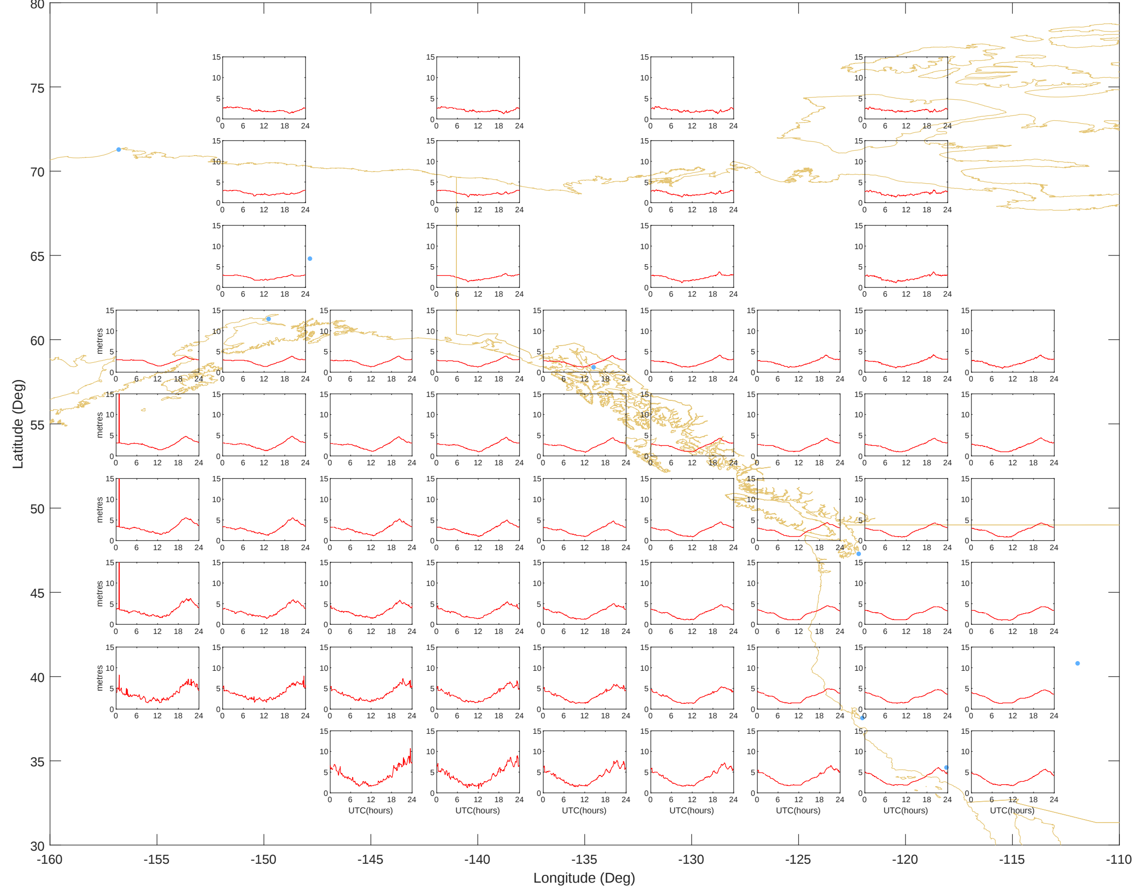
Ionospheric Grid Delays - Alaska (13-May-2025) @UNB-WAASLAB
