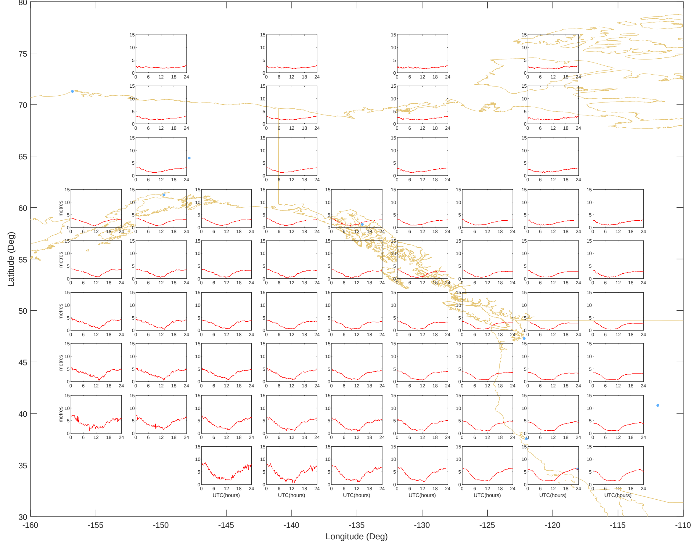
Ionospheric Grid Delays - Alaska (10-May-2025) @UNB-WAASLAB
