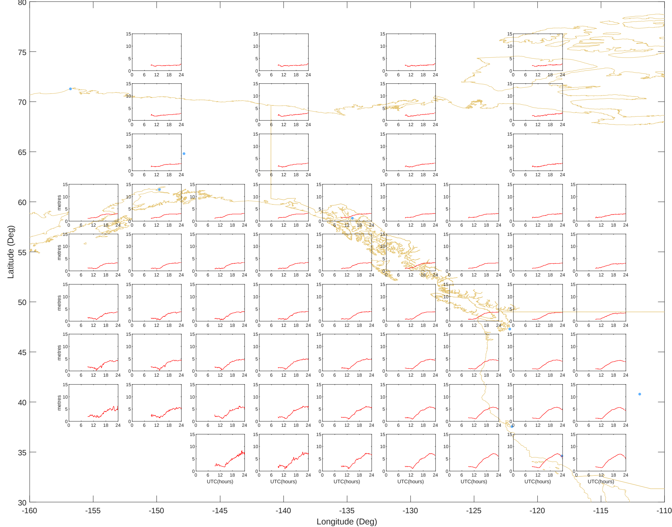
Ionospheric Grid Delays - Alaska (07-May-2025) @UNB-WAASLAB
