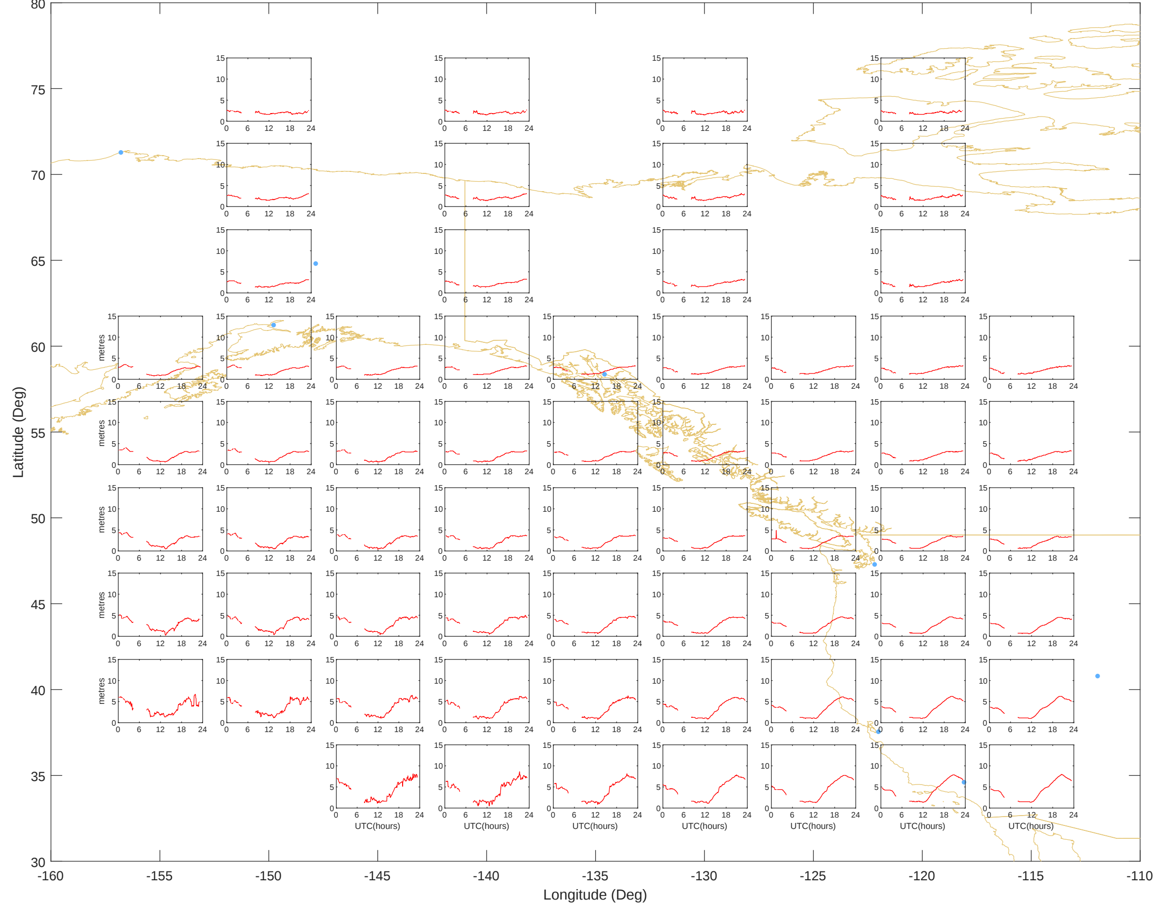
Ionospheric Grid Delays - Alaska (06-May-2025) @UNB-WAASLAB
