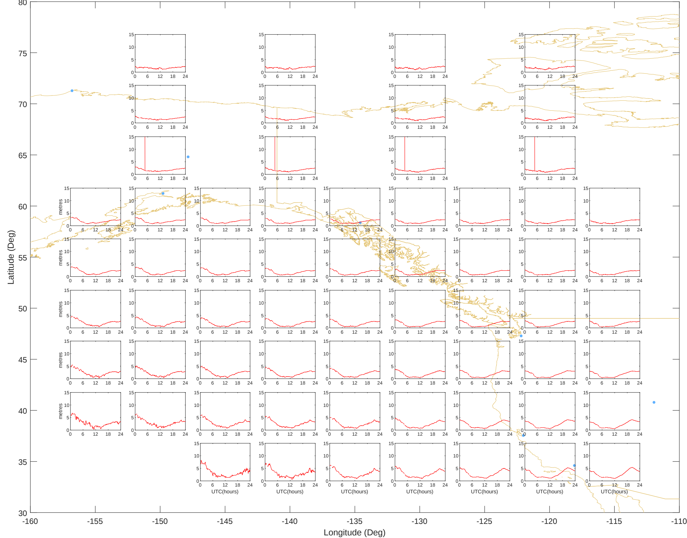
Ionospheric Grid Delays - Alaska (03-May-2025) @UNB-WAASLAB
