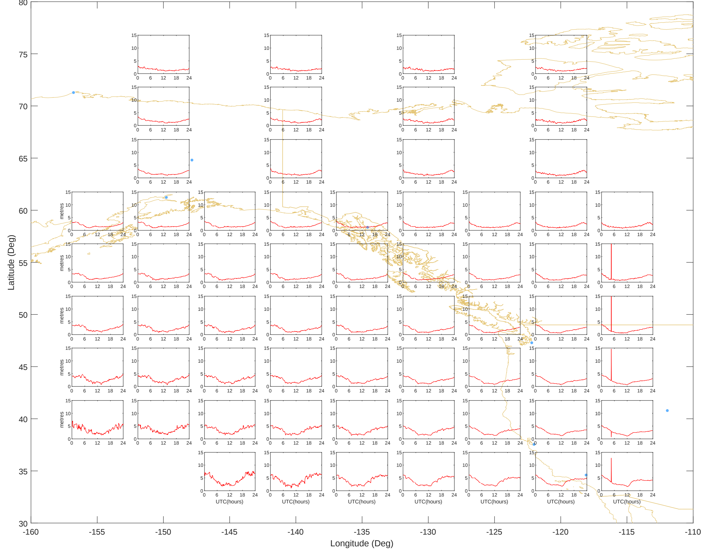
Ionospheric Grid Delays - Alaska (02-May-2025) @UNB-WAASLAB
