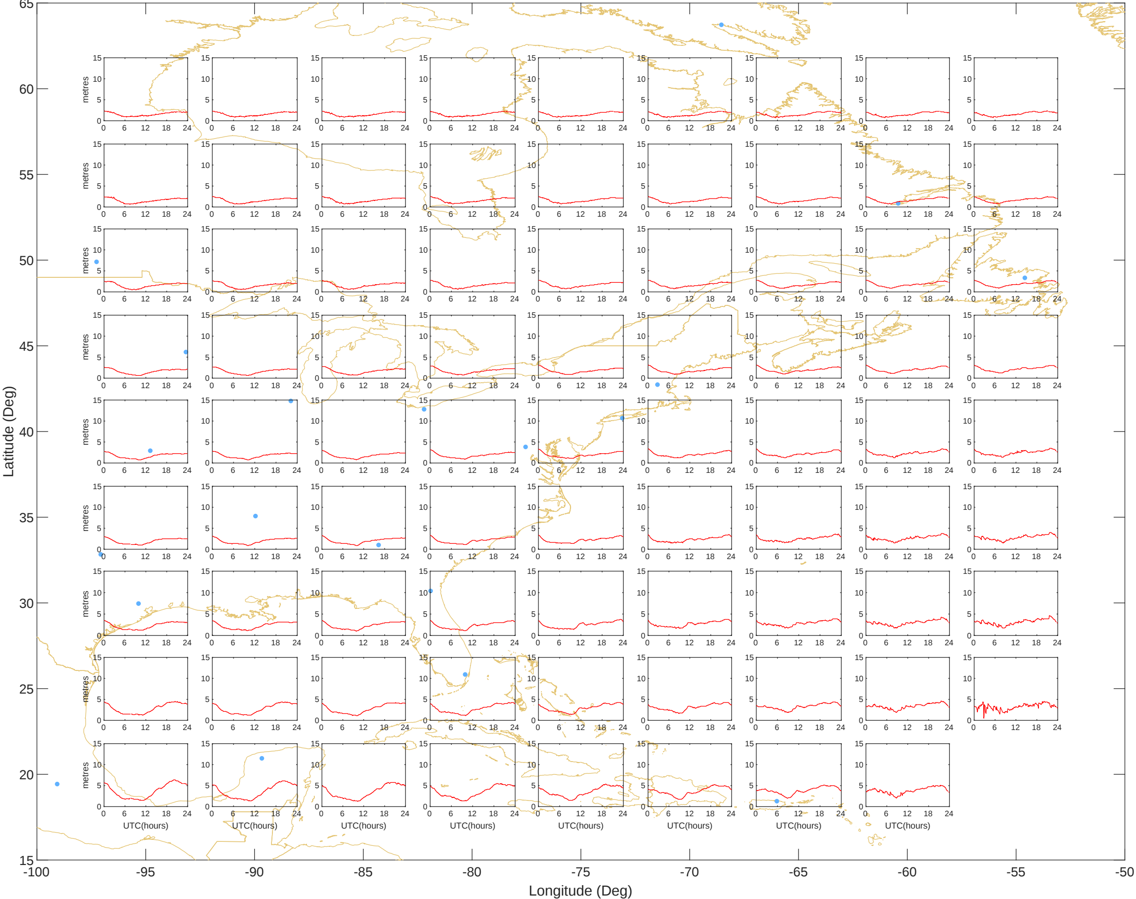
Ionospheric Grid Delays - East (12-Jul-2026) @UNB-WAASLAB
