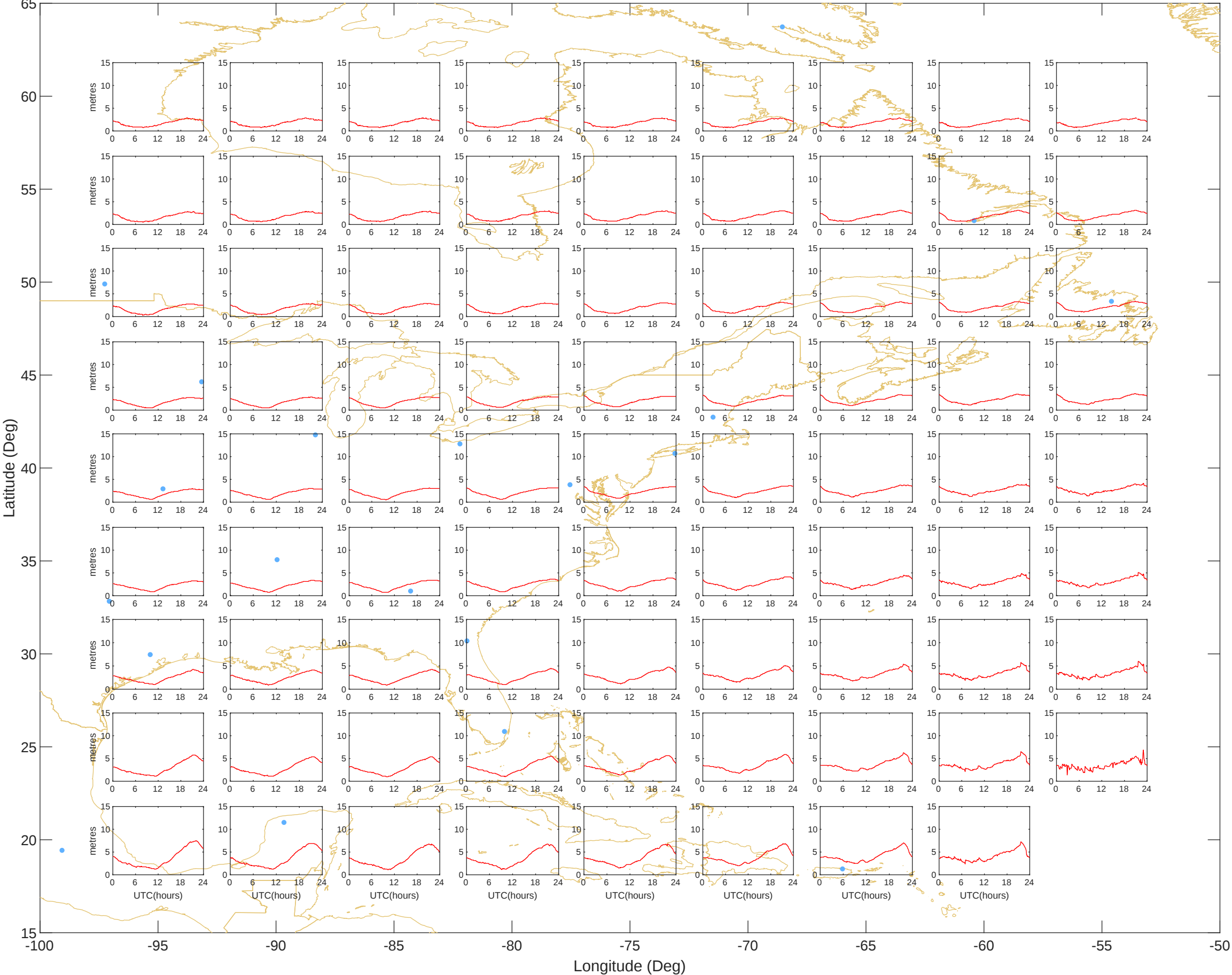
Ionospheric Grid Delays - East (11-Jul-2026) @UNB-WAASLAB
