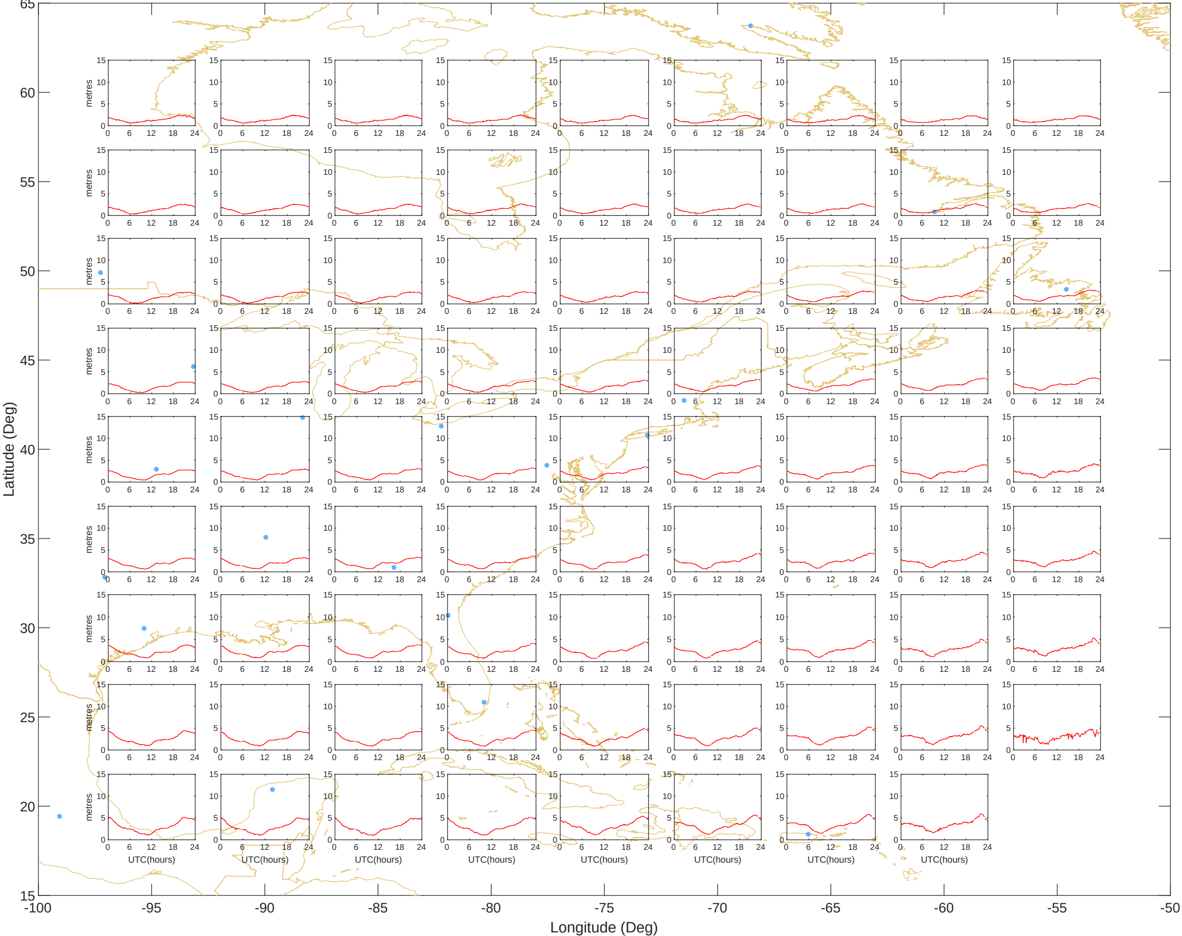
Ionospheric Grid Delays - East (09-Jul-2026) @UNB-WAASLAB
