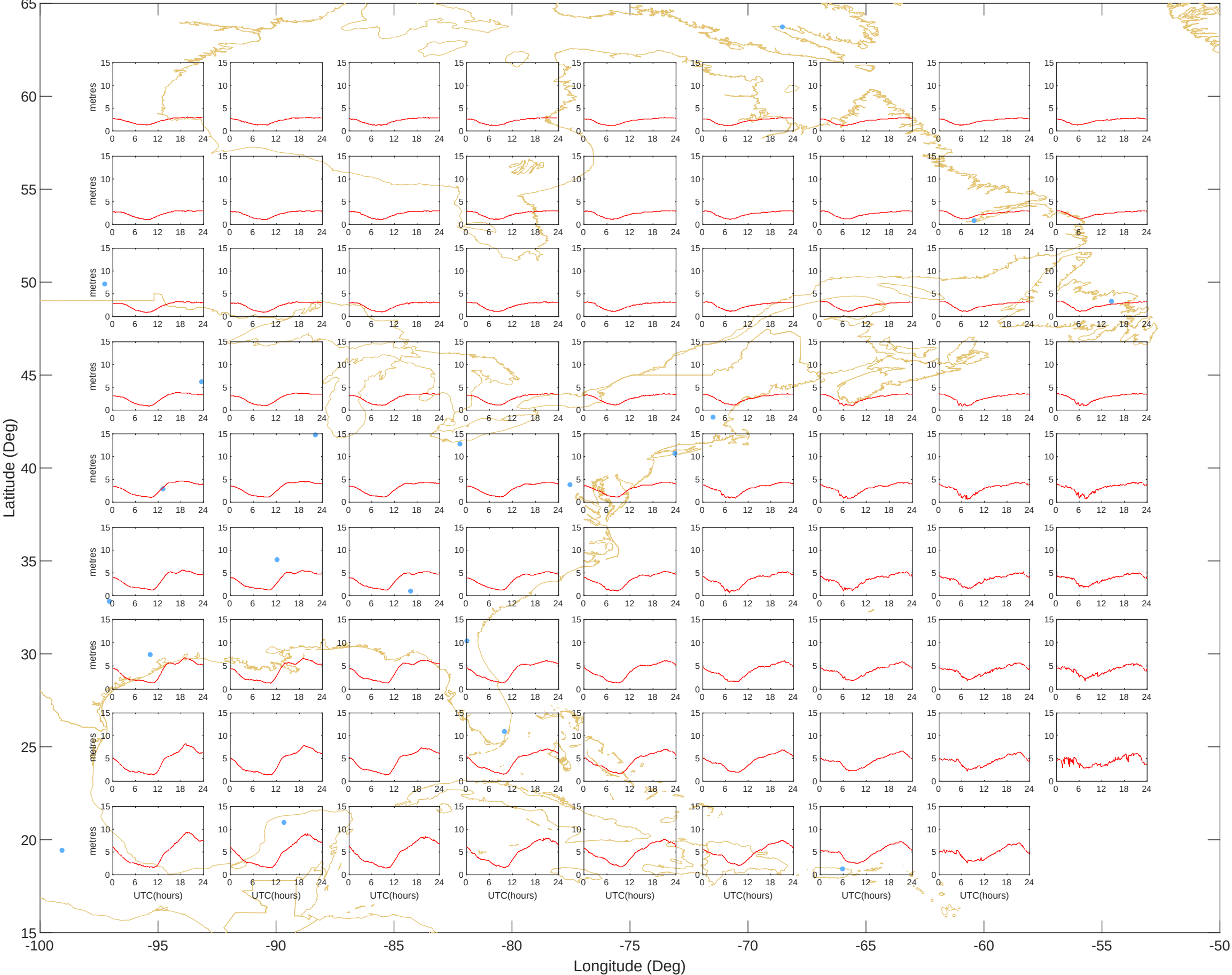
Ionospheric Grid Delays - East (02-Jul-2026) @UNB-WAASLAB
