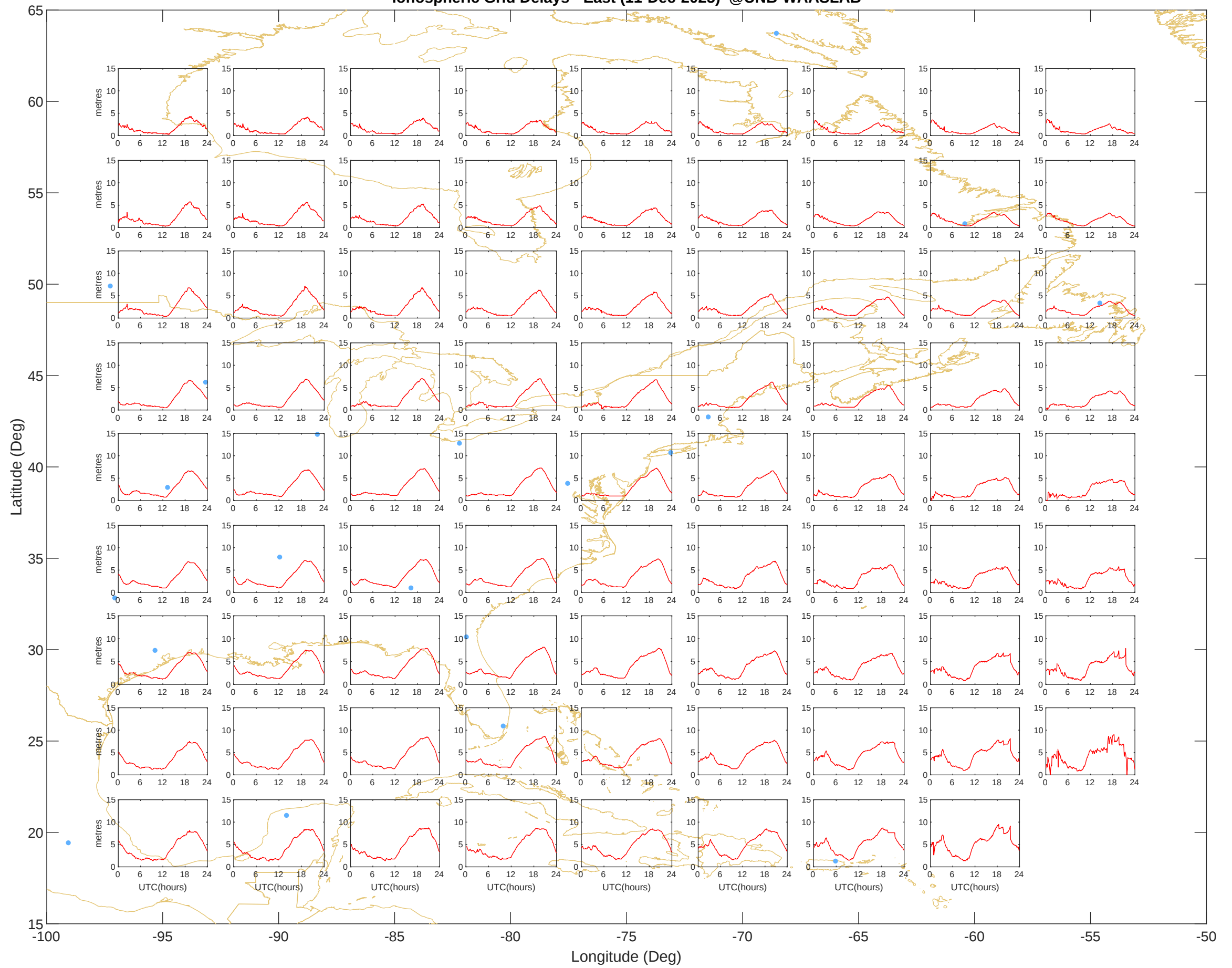
Ionospheric Grid Delays - East (11-Dec-2025) @UNB-WAASLAB
