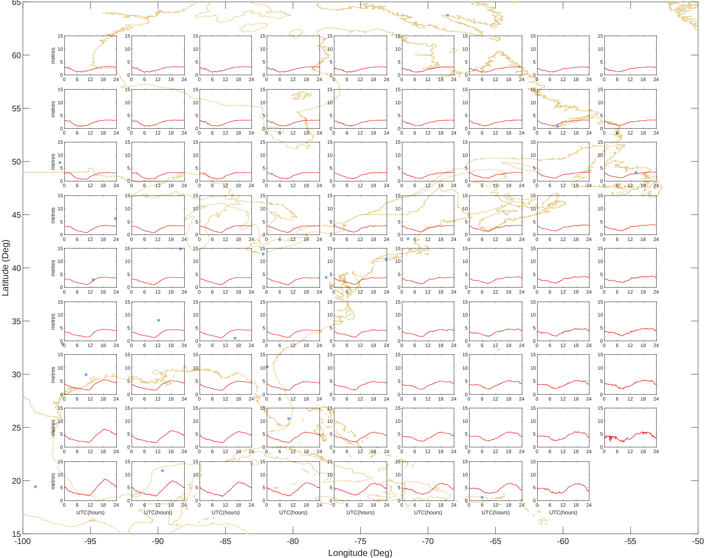
Ionospheric Grid Delays - East (29-Jul-2025) @UNB-WAASLAB
