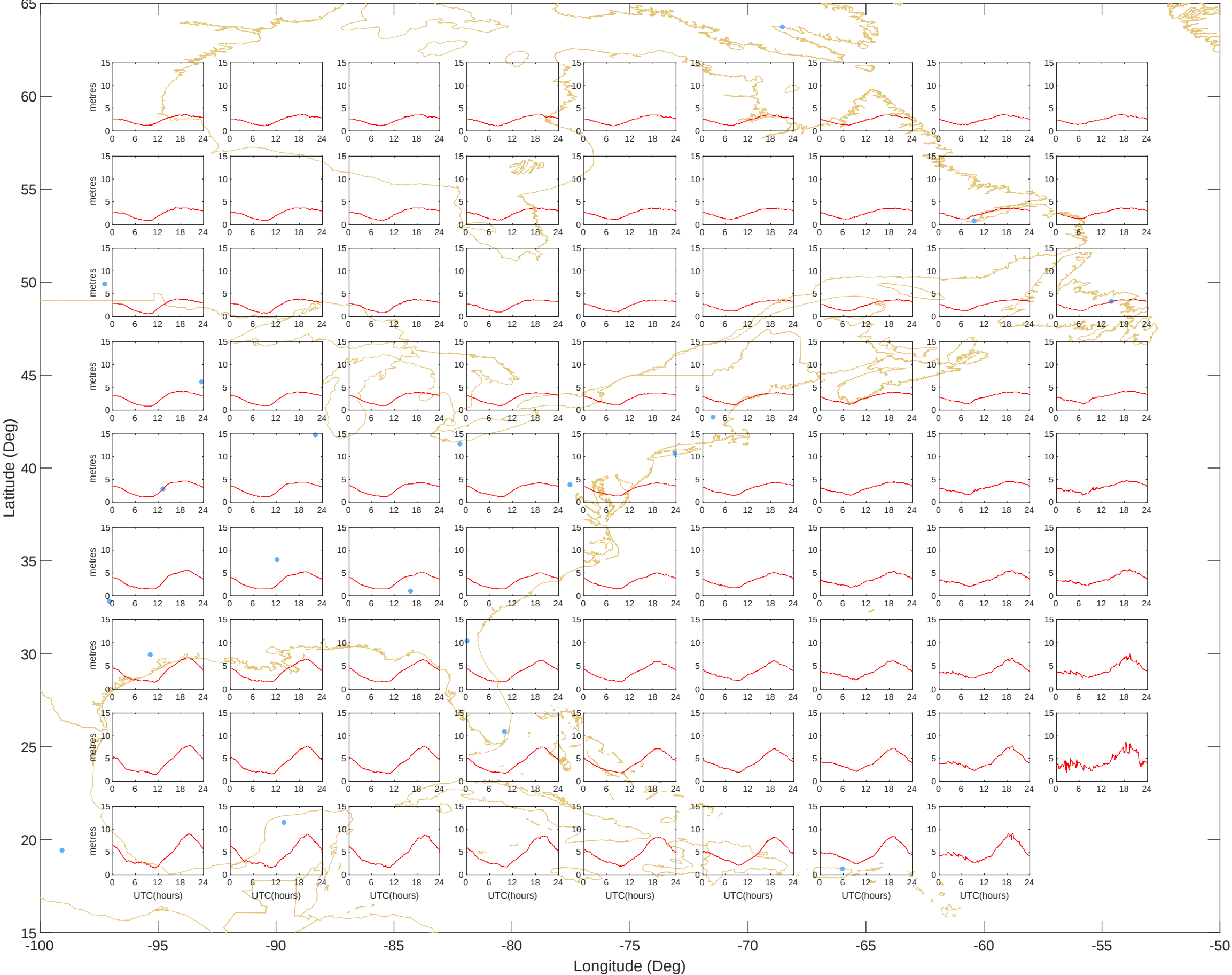
Ionospheric Grid Delays - East (28-Jul-2025) @UNB-WAASLAB
