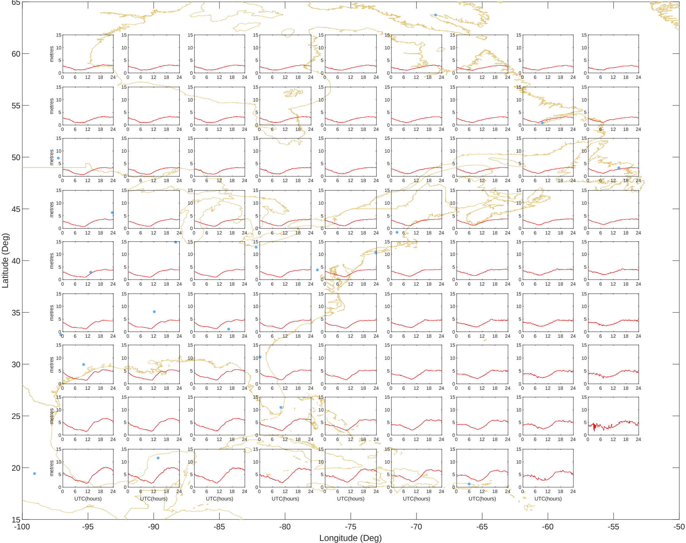
Ionospheric Grid Delays - East (25-Jul-2025) @UNB-WAASLAB
