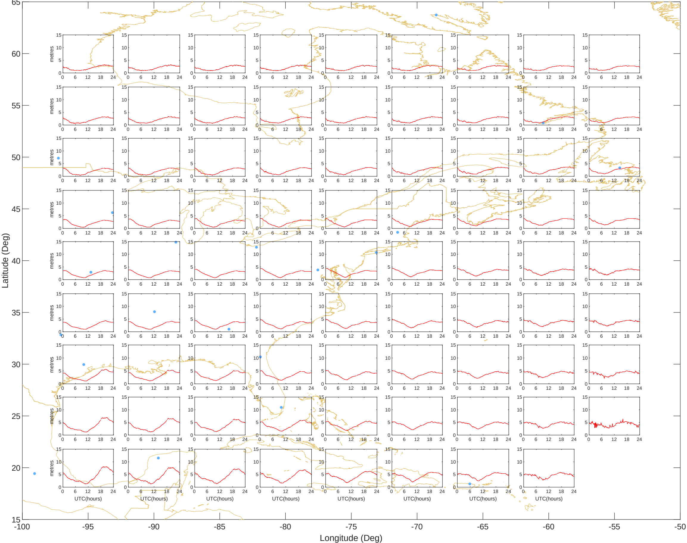
Ionospheric Grid Delays - East (24-Jul-2025) @UNB-WAASLAB
