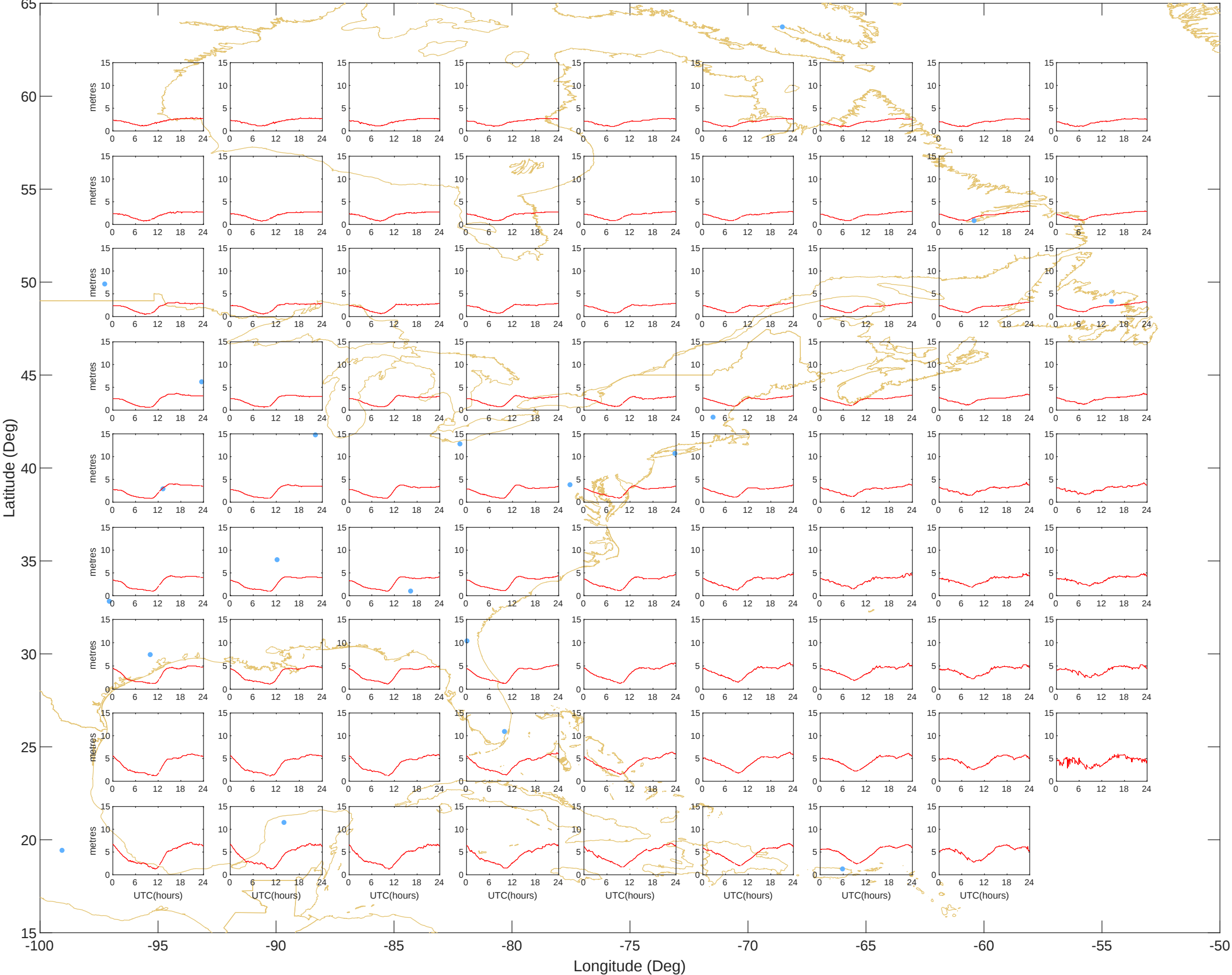
Ionospheric Grid Delays - East (20-Jul-2025) @UNB-WAASLAB
