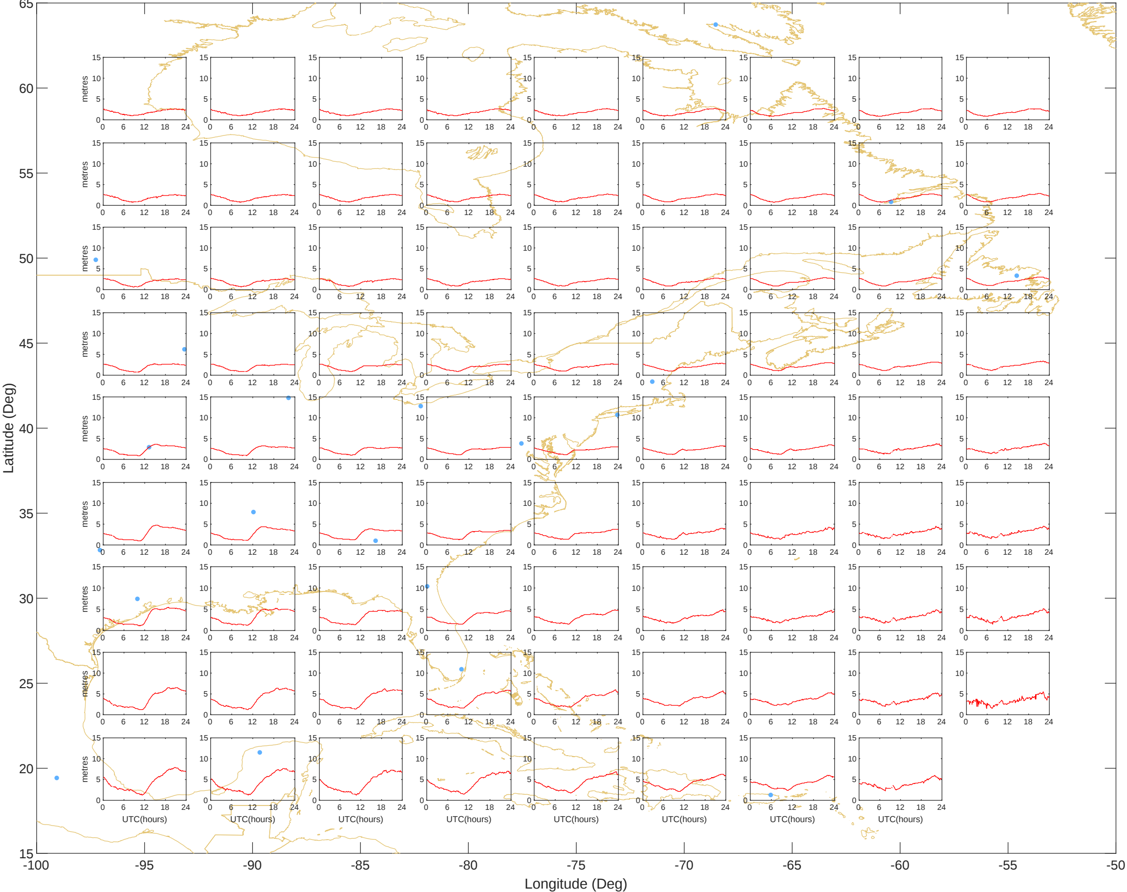
Ionospheric Grid Delays - East (19-Jul-2025) @UNB-WAASLAB
