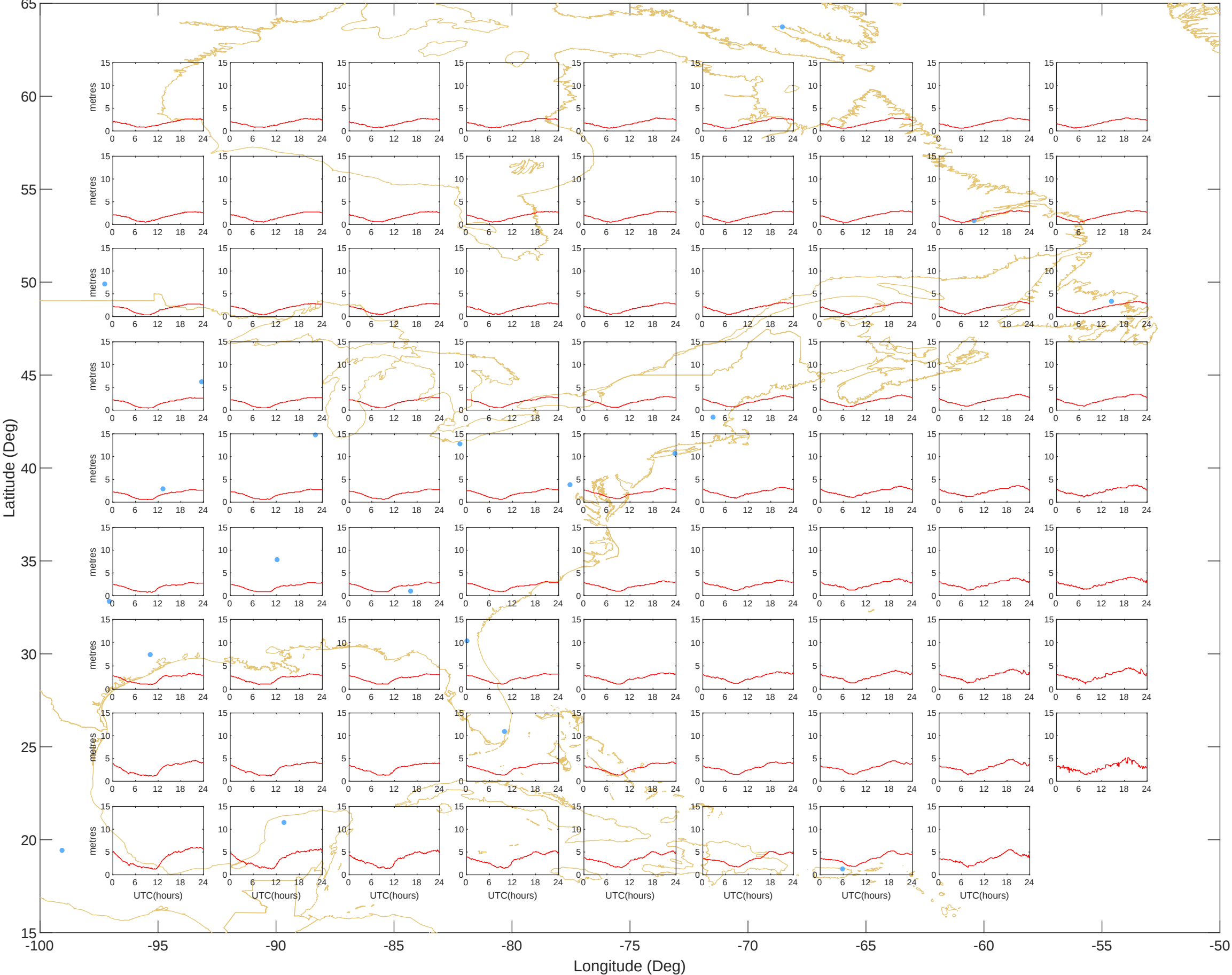
Ionospheric Grid Delays - East (18-Jul-2025) @UNB-WAASLAB
