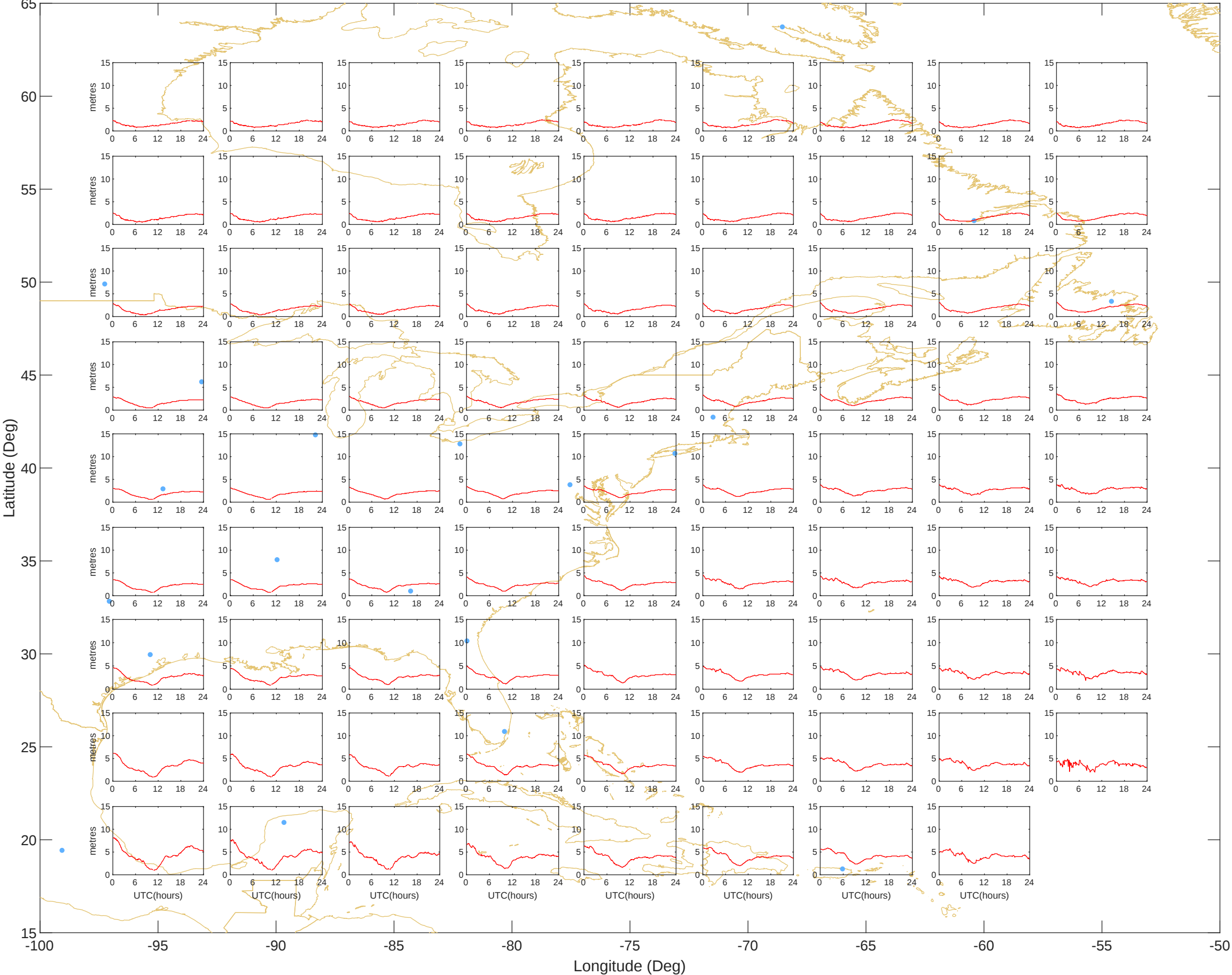
Ionospheric Grid Delays - East (17-Jul-2025) @UNB-WAASLAB
