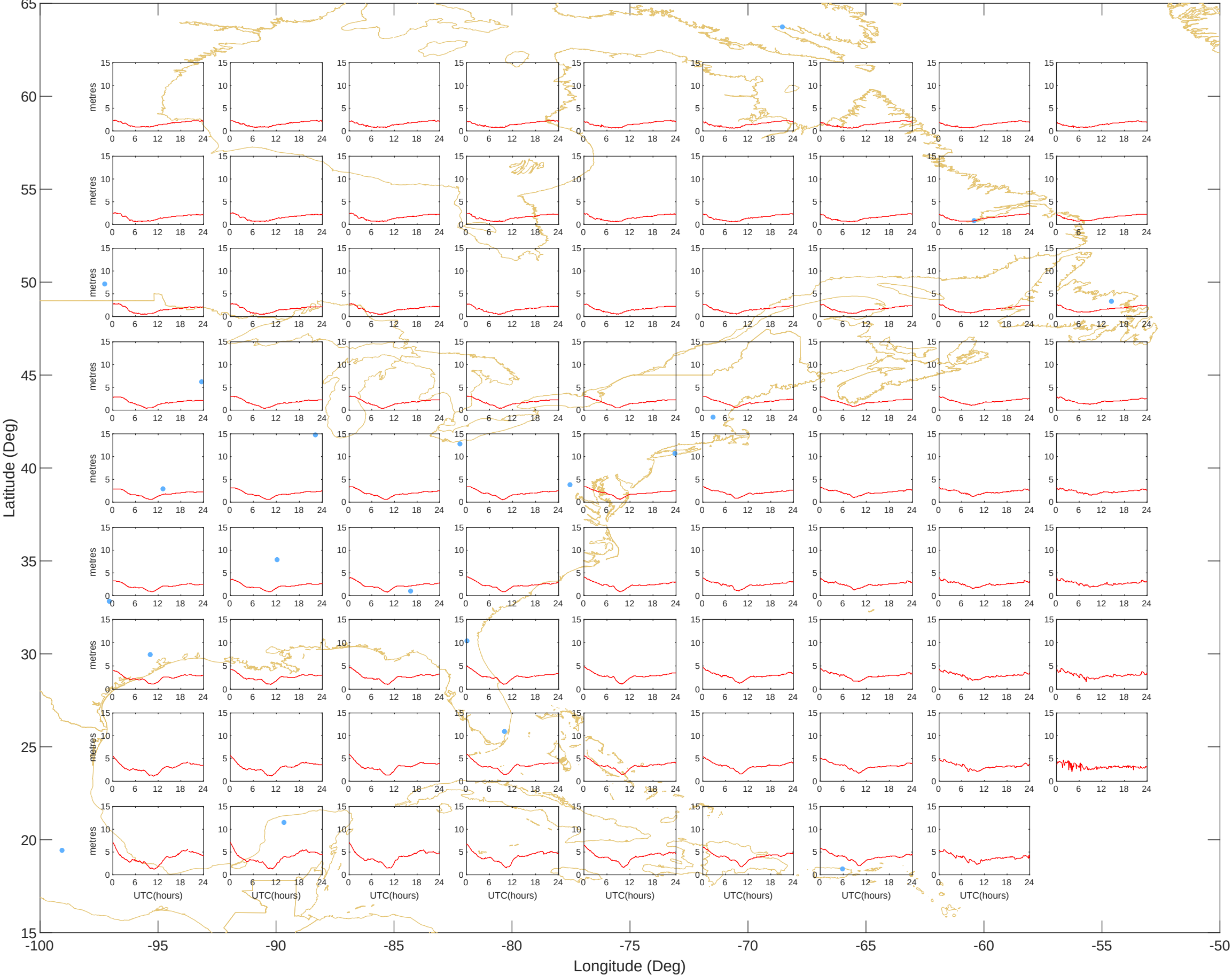
Ionospheric Grid Delays - East (15-Jul-2025) @UNB-WAASLAB
