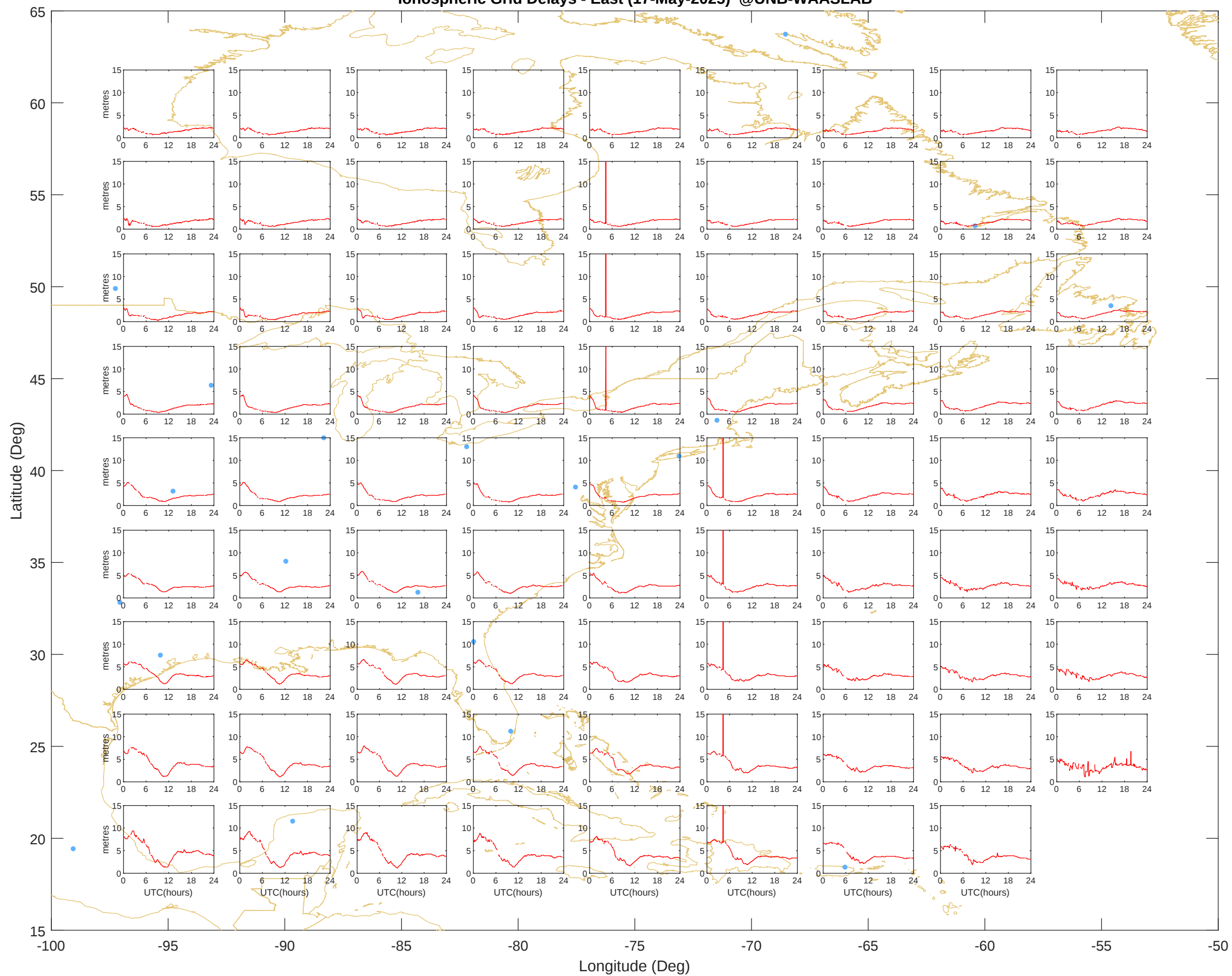
Ionospheric Grid Delays - East (17-May-2025) @UNB-WAASLAB
