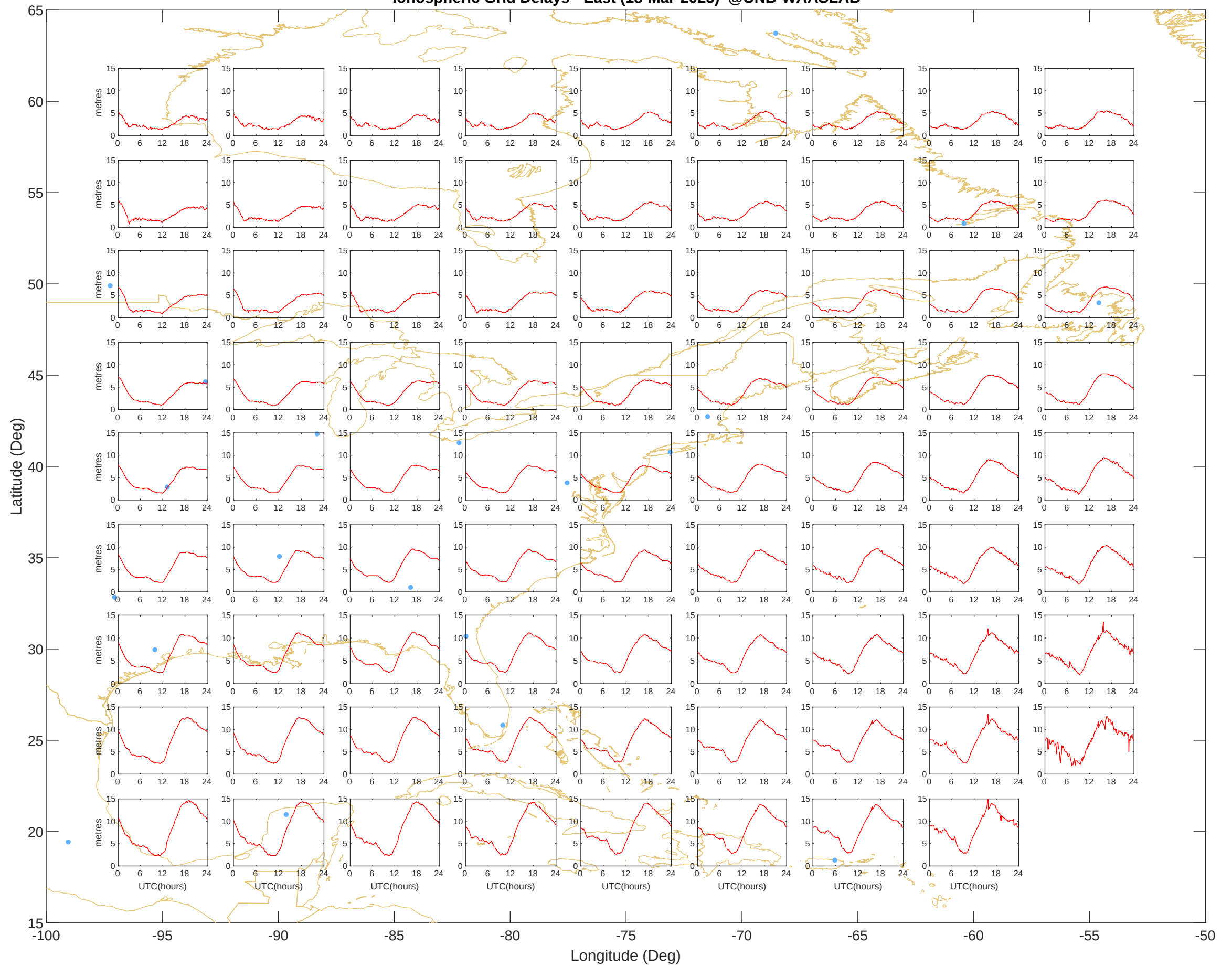
Ionospheric Grid Delays - East (18-Mar-2025) @UNB-WAASLAB
