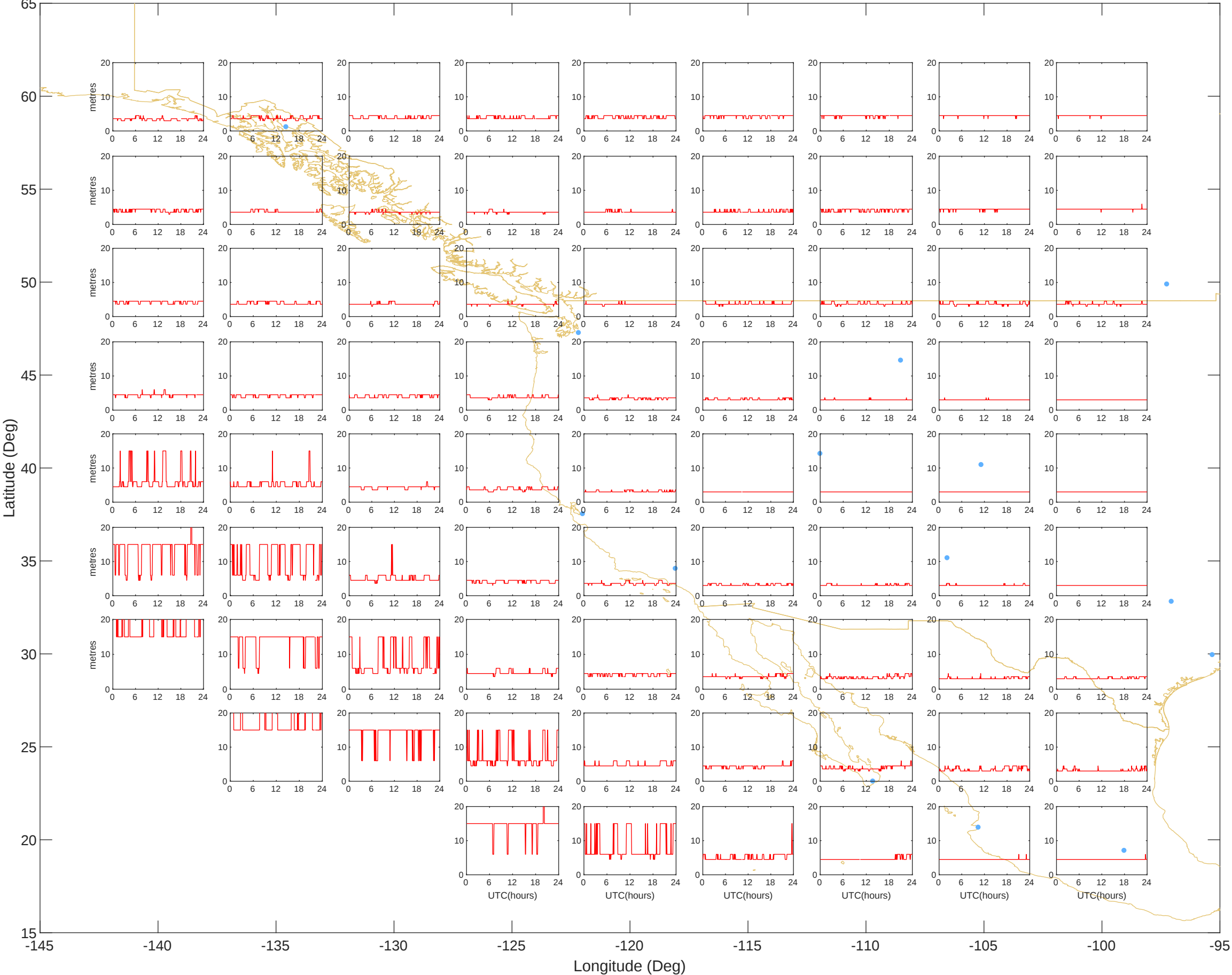
GIVES - West (16-Jul-2025) @UNB-WAASLAB
